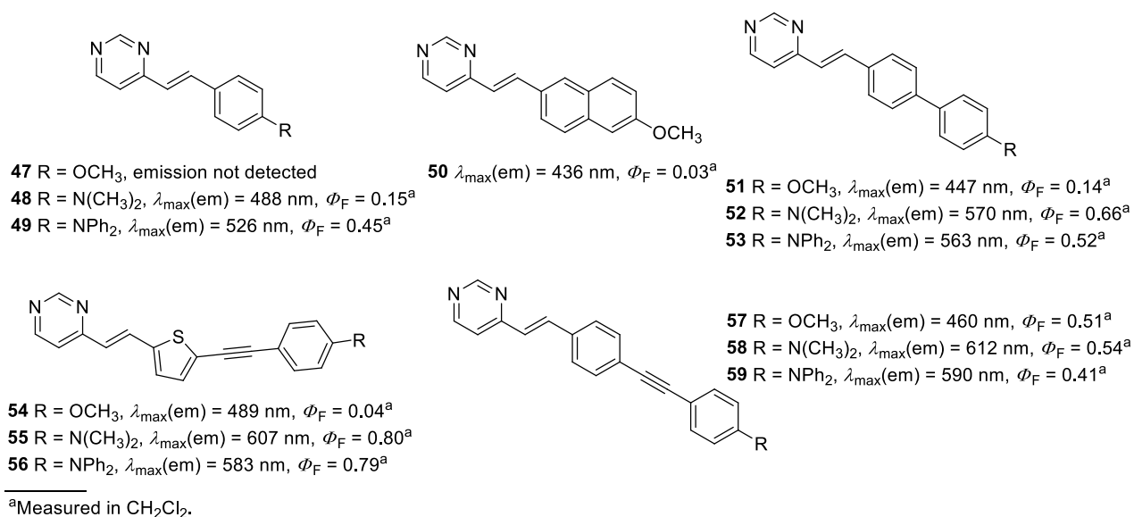
Figure 25. PL properties of compounds 47–59 with gradually extended conjugated pathway.
