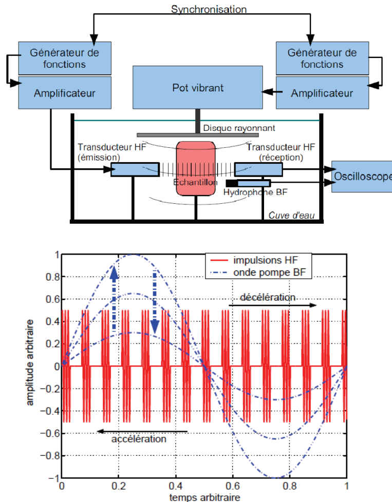
Figure 137 : Principe de la technique DAET [Ren08]
