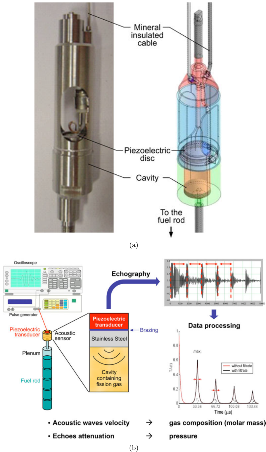
Figure 8.2 – (a) Acoustic sensor designed to be implemented on sample fuel rod to be irradiated in research reactor. (b) Principle of acoustic sensor for fission gas release measurement [Kim11]
