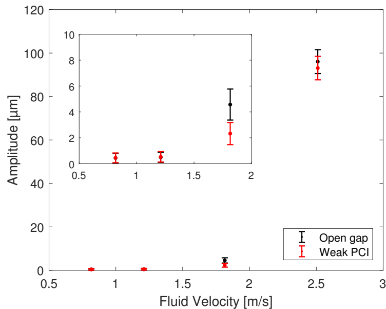
Figure 11.11 – Root Mean Square amplitude of flow induced vibrations for the C3 fuel rod, k=1
