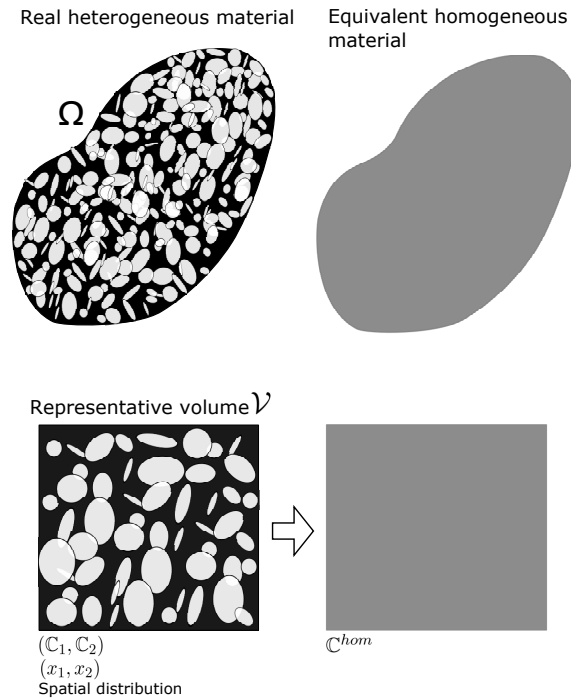
Figure 5.1 – Homogenization principle
