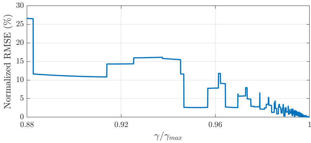
Figure 4.7: Normalized RMSE, \sqrt{\sum_i f_i(\mathbf{n}, \gamma)^2 / \ell} for different values of \gamma .
