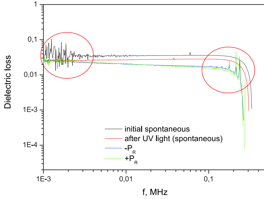
Figure 2.3: Example of the frequency dependence of dielectric loss in the sample recorded for different polarization states.
