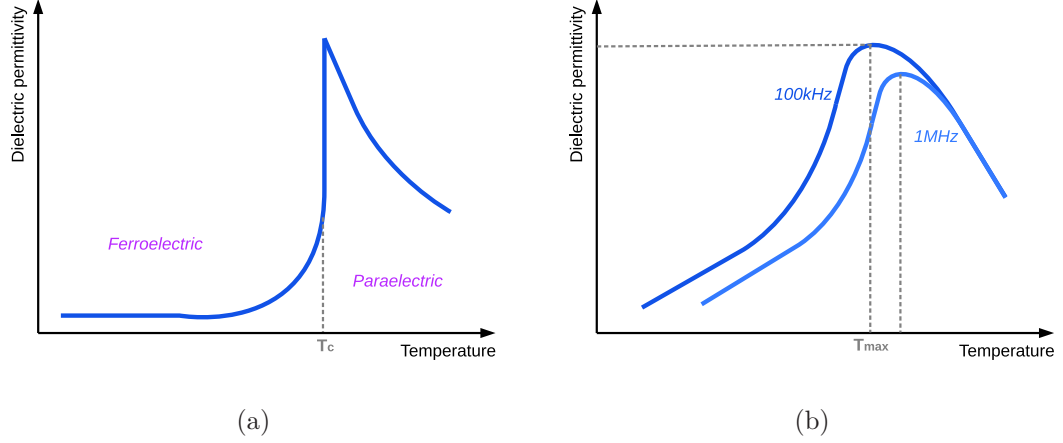
Figure 1.7: Schematic representation of dielectric permittivity as a function of temperature in "normal" (a) and relaxor (b) ferroelectrics.
