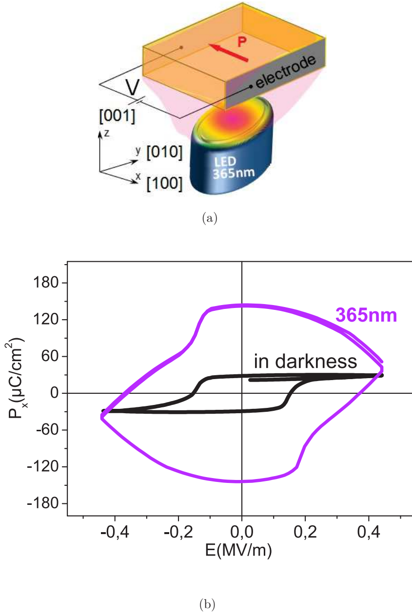
Figure 3.8: Schematic of the measurements with respect to crystal axis (a). The FE loop of the PMN-PT30% measured in darkness and under UV light (b).
