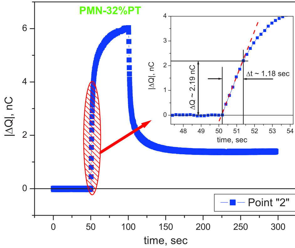
Figure 3.7: Charges generation efficiency in PMN-PT32% composition. Note that the linear part was taken for efficiency calculations.
