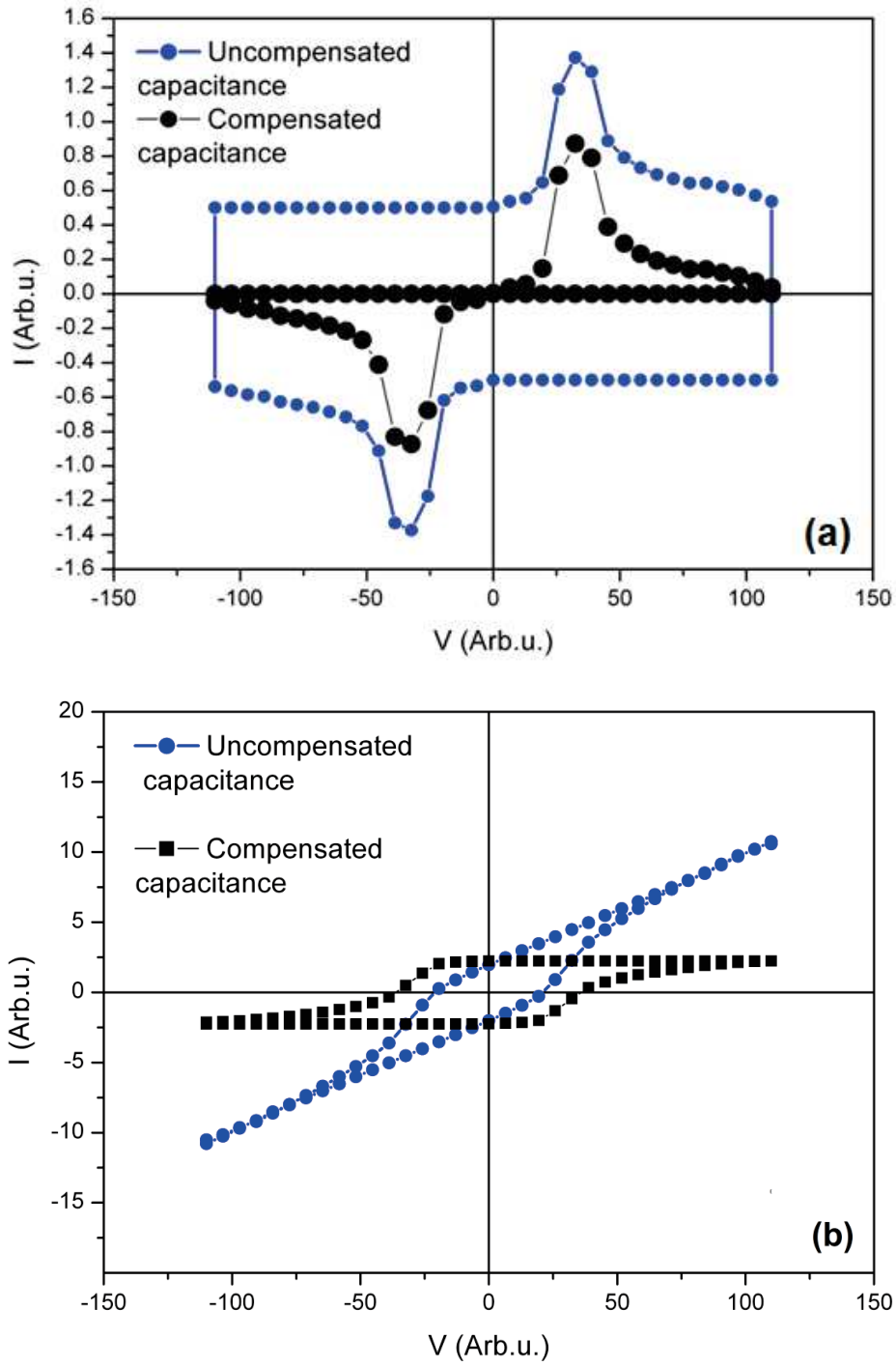
Figure 2.8: Example of the I-V characteristic recorded on a background large linear capacitance contribution before (a) and after (b) capacitance compensation.
