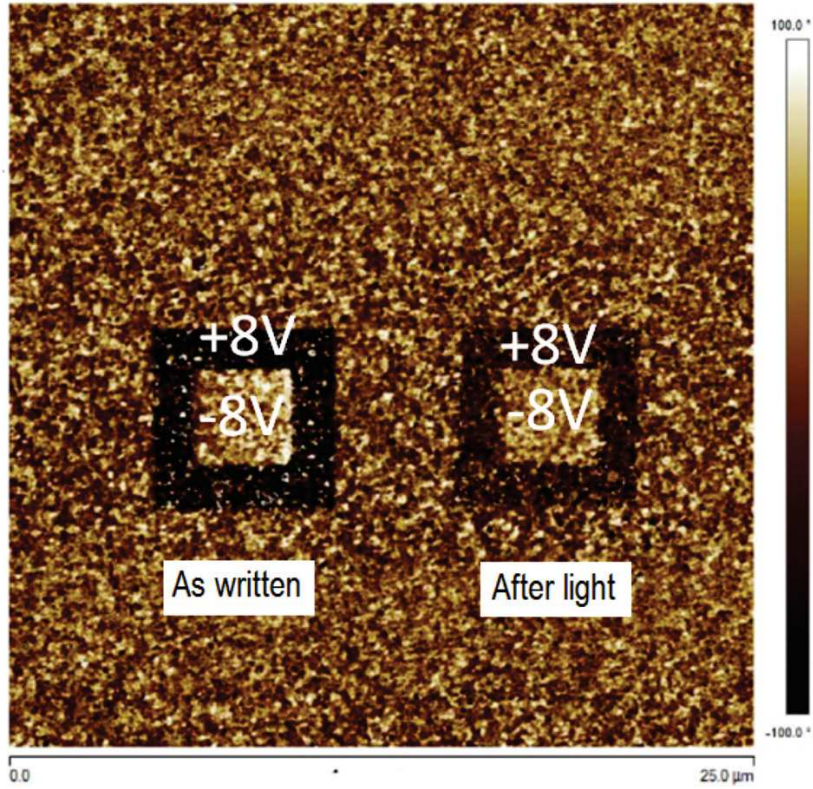
Figure 3.18: PFM poling (phase) images before and after exposure to 365\text{ nm} light.
