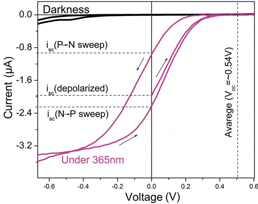
Figure 3.16: Current-voltage measurements on a BFCO sample, in darkness and under 365\text{ nm} light irradiation.
