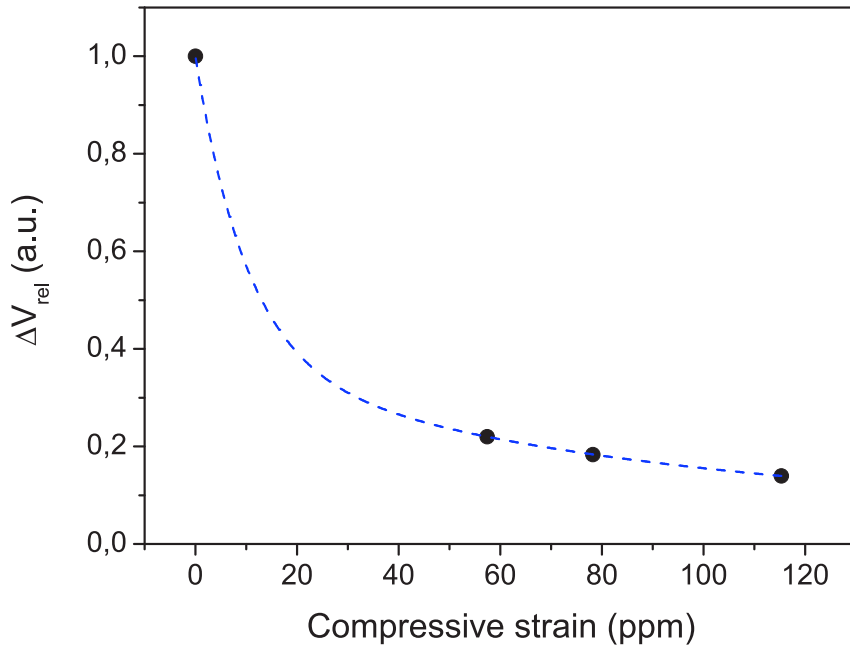
Figure 6.4: PMN-PT30% photovoltaic effect tuning by compressive strain (ppm defined in Eq. (2.17)).
