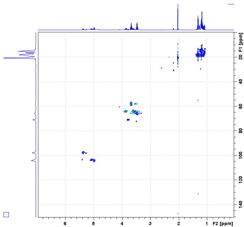
Figure 57. Spectre HSQC ^1\text{H} - ^{13}\text{C} de la Fraction FC732
