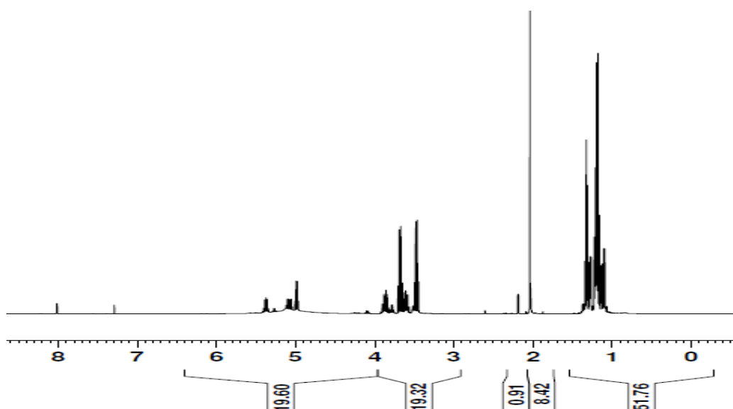
Figure 54. Spectre RMN ^1\text{H} (400 MHz, \text{CDCl}_3 ) de la Fraction FC732
