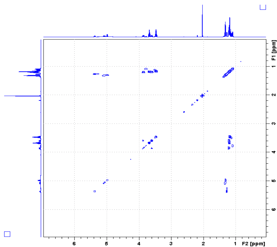
Figure 56. Spectre COSY ^1\text{H} - ^1\text{H} de la Fraction FC732
