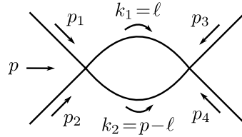
Figure 2.1 – 1-loop 4-point function for a scalar field theory.
