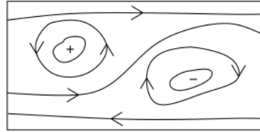
FIGURE 2.5: The localisation of states due to disorder. The drawn lines correspond to equipotentials.
