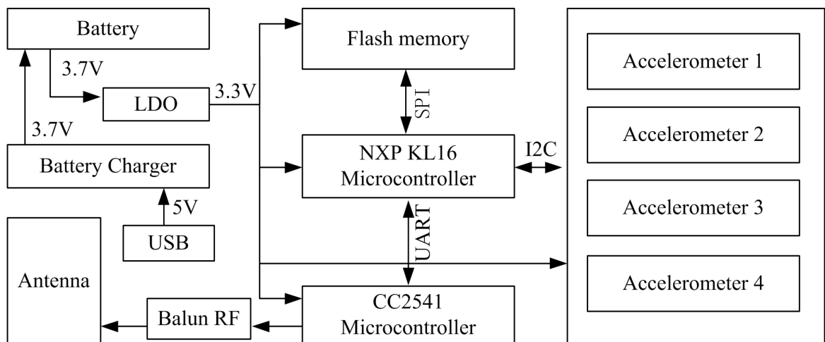
(a) Block circuit diagram of the intelligent garment hardware.
