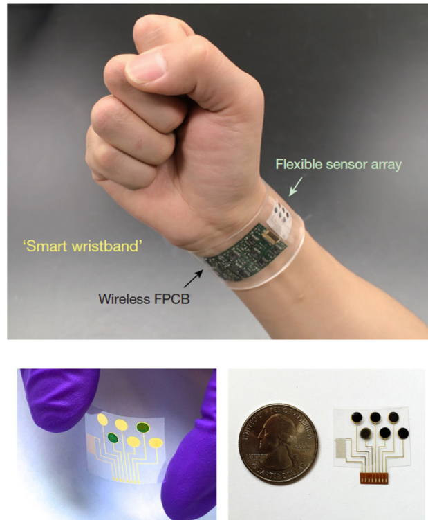
Figure 1.8 – A smart wristband integrating flexible sensors presented in [Gao et al. (2016)].
