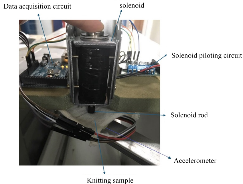
Figure 3.2 – Testing of signal attenuation of different fabrics using a solenoid.
