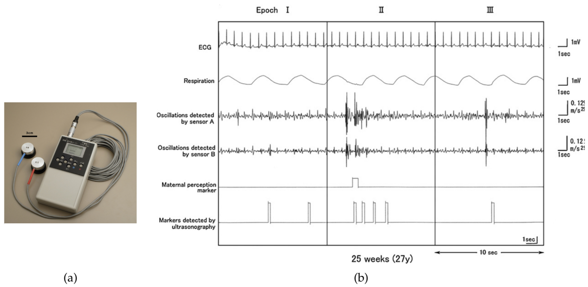
Figure 1.4 – (a) An accelerometer-based fetal movement recorder together with (b) an example of acquired signals using the recorder (only acceleration signals on z-axis were studied and illustrated) with other physiological signals e.g. maternal ECG and respiration (adapted from [Ryo et al. (2012)]).
