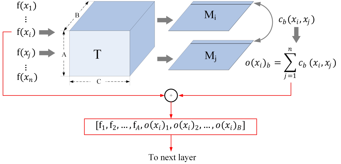
Figure 6.4 – Minibatch discrimination.
