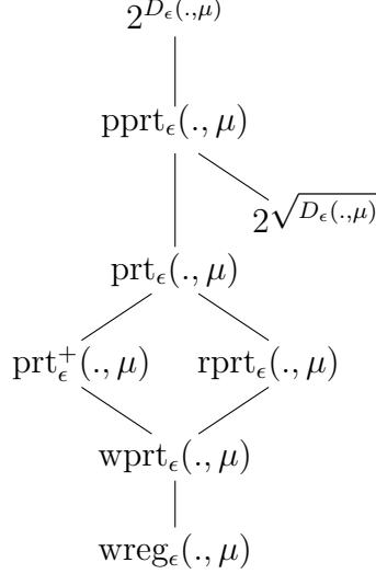
Figure 9: Relations between bounds in their distributional versions. A similar diagram appears in [FJK + 16].
