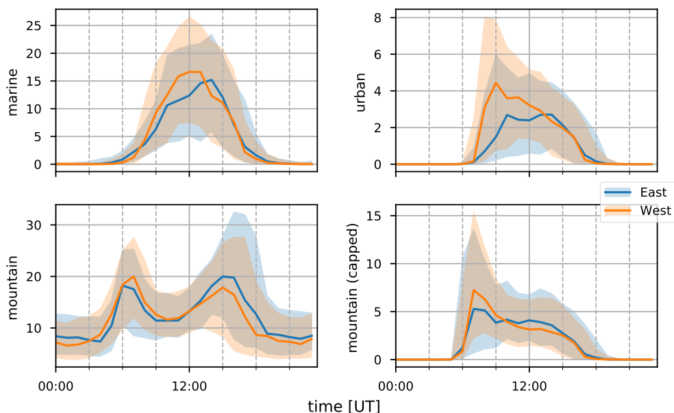
Diel cycle of SRRs [ \text{s m}^{-1} ]
