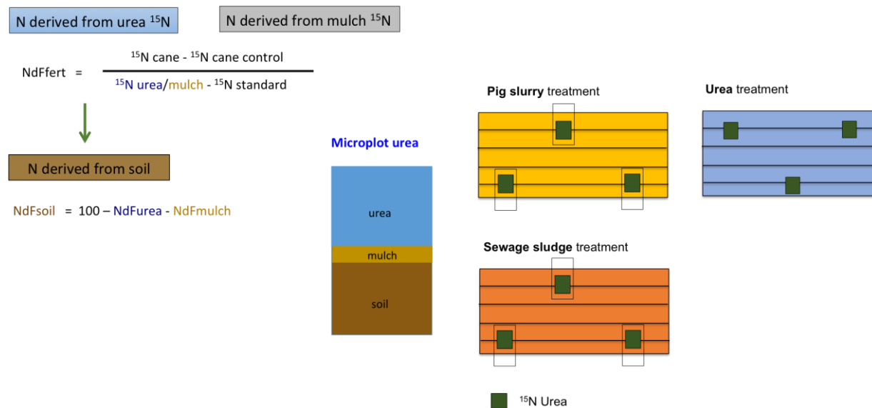
Figure 9. Calculation of nitrogen derived from 15 N enriched urea, 15 N enriched mulch, and from the soil as calculated by deduction.
