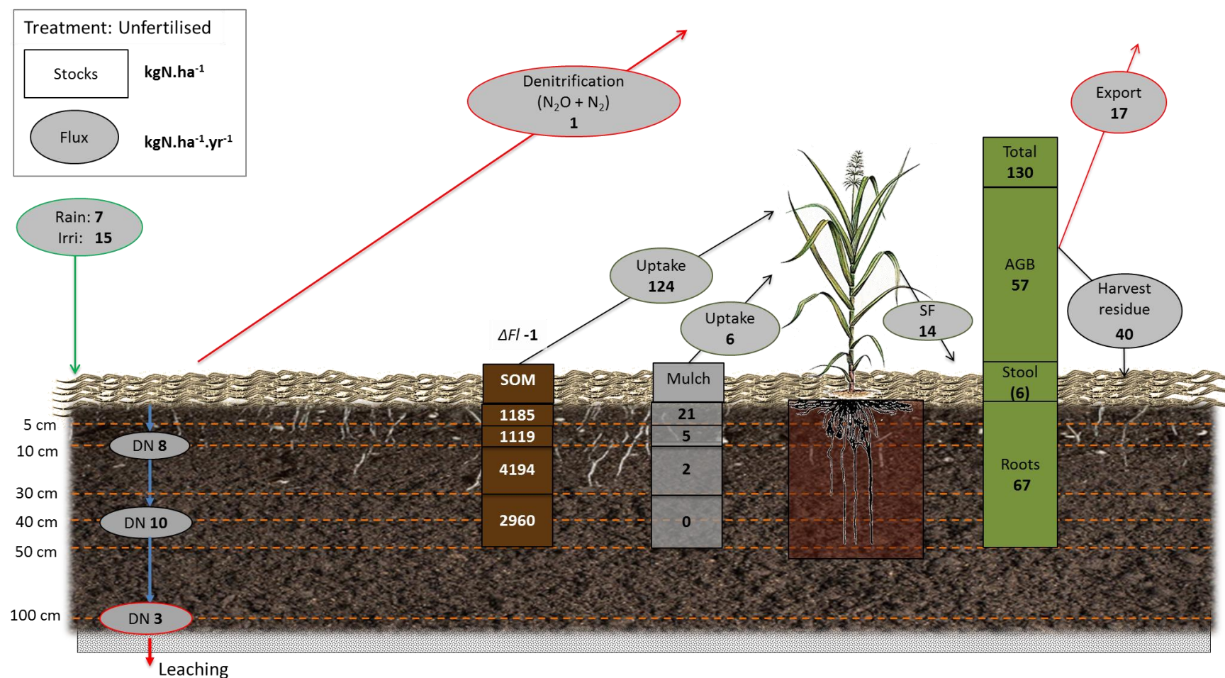
Figure 5.1 Nitrogen budget for the unfertilised treatment, averaged over the two experimental years. Summarised are the N inputs of rainfall (Rain) and irrigation (Irr), and sugarcane green tops and straw left after harvest (Harvest Residue), and strawfall (SF) that falls to the soil over the sugarcane growth-cycle. The outputs of harvested sugarcane (Export), N emitted in the form of \text{N}_2\text{O} and \text{N}_2 gases via denitrification (Denitrification), dissolved nitrogen in soil solution (DN), with the portion at a soil depth of 100 cm lost from the soil-sugarcane system via leaching. The stocks of soil organic matter (SOM) and mulch (Mulch) and the relative uptake (Uptake) of these sources by the sugarcane are displayed. The N stocks in the different compartments of the sugarcane are shown, in the aboveground biomass (AGB), the stools (Stools), roots (Roots) and total N for the entire plant (Total).
