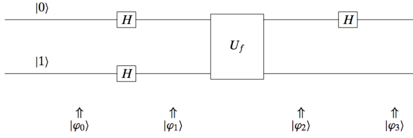
FIGURE 1.11: Deutsch Jozsa circuit
