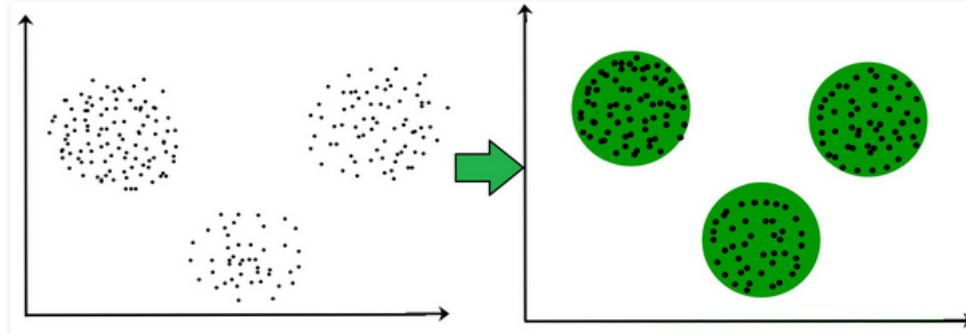
FIGURE 3.1: Clustering
