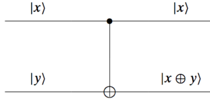
FIGURE 1.6: C-Not gate
