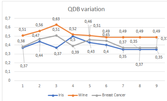
FIGURE 3.19: QDavies-Bouldin Variation
