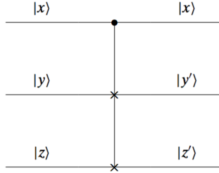
FIGURE 1.8: Fredkin gate
