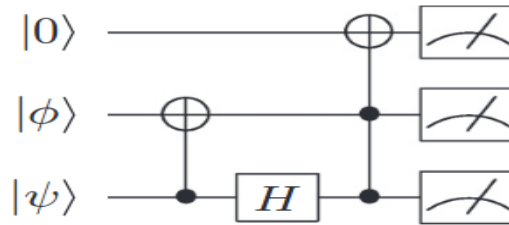
FIGURE 3.7: Rewriting CCZ as CCNOT
