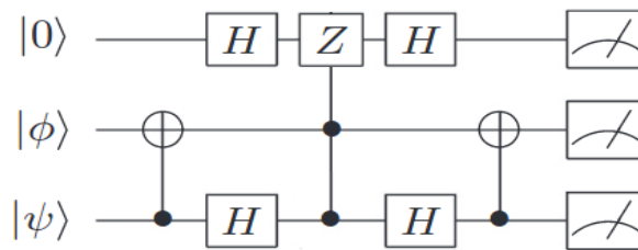
FIGURE 3.5: Symmetry of CCZ
