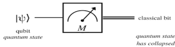
FIGURE 1.10: Measurement
