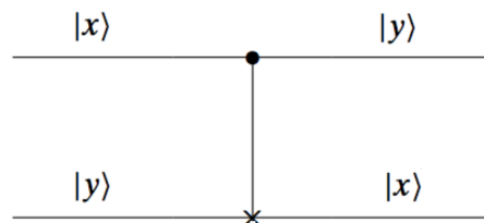
FIGURE 1.7: Swap Gate
