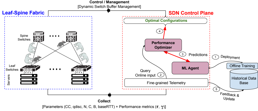
Figure 6.2: SDN-enabled ML-based Smart Buffer Management Framework
