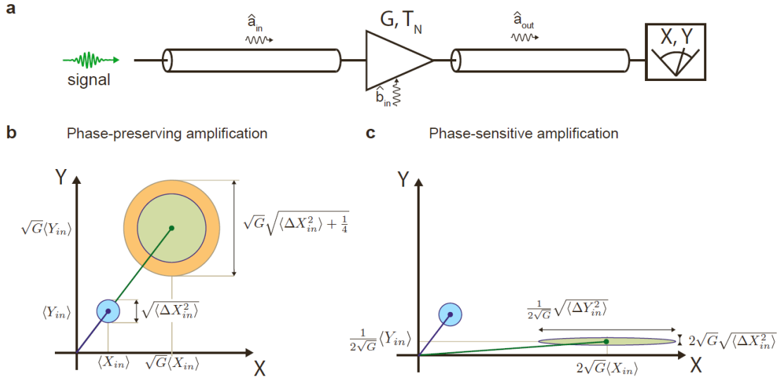
Figure 2.7: Linear amplifiers. (a) A linear amplifier of gain G and noise temperature T_N is used to detect a narrow-band signal. (b)-(c) Phase-preserving and phase-sensitive amplification in phase-plane representation in the limit of high gain. The disks indicate the contour of the Wigner function. A phase preserving amplifier degrades the SNR, with the added noise represented in red. In phase-sensitive amplification, one quadrature is amplified at the expense of the other, but one can evade the noise added by the Heisenberg uncertainty principle.
