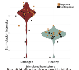
Fig. 6 Hallucinatory excitability
