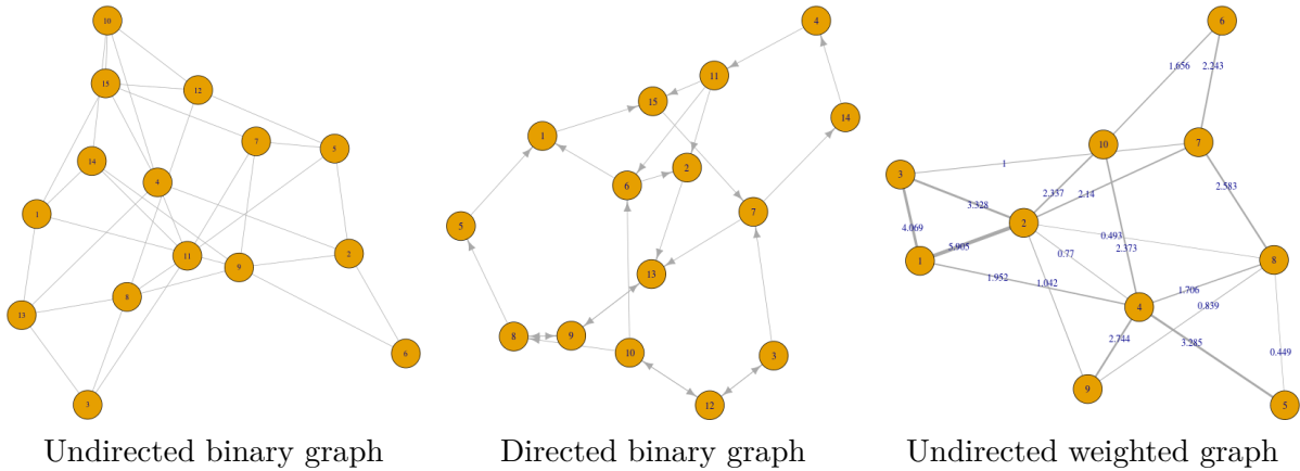
Fig. 1.1 Representation of different types of graphs
