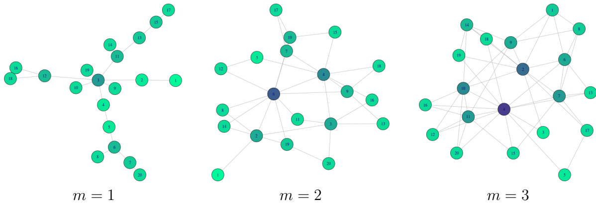
Fig. 1.3 Barabási–Albert model for different values of m , all starting from an initial graph of 5 nodes.
