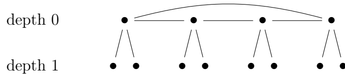
Fig. 1.1. An \ell -volcano with \ell = 3 , d_{\max} = 1 , and \left(\frac{\Delta}{\ell}\right) = 1 .
