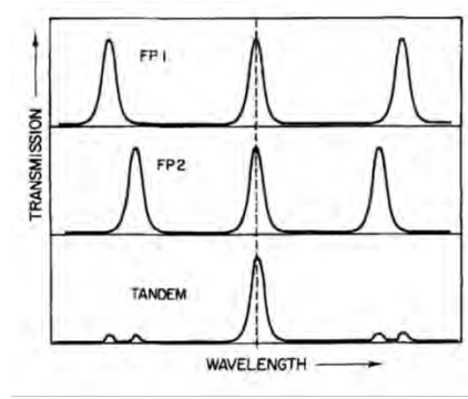
Figure 2.29 – Transmission of light within each Fabry Pèrot (FP) and in tandem operation after superposition of one transmission order for each.
