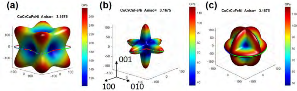
Figure 4.1 - Orientation dependence of (a) Young's modulus E , (b) minimum shear modulus, (c) maximum shear modulus G , for CoCrCuFeNi . The input elastic constants were calculated by VASP-SQS, considering FM state and atomic positions relaxations.
