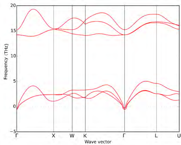
Figure A.5 - The phonon dispersion curves of Ta_4N_3 with Pm\bar{3}m symmetry.
