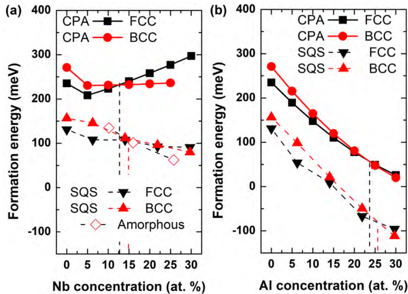
Figure 5.1 - Formation energy calculated by EMT0-CPA and VASP-SQS for (a) (\text{CoCrCuFeNi})_{1-x}\text{Nb}_x and (b) (\text{CoCrCuFeNi})_{1-x}\text{Al}_x with FCC, BCC and amorphous structures. The energy cross between different structures is indicated by vertical dashed lines.
