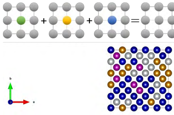
Figure 2.2 - Schematic illustration of the coherent potential approximation (above), below is a supercell used to calculate random materials.
