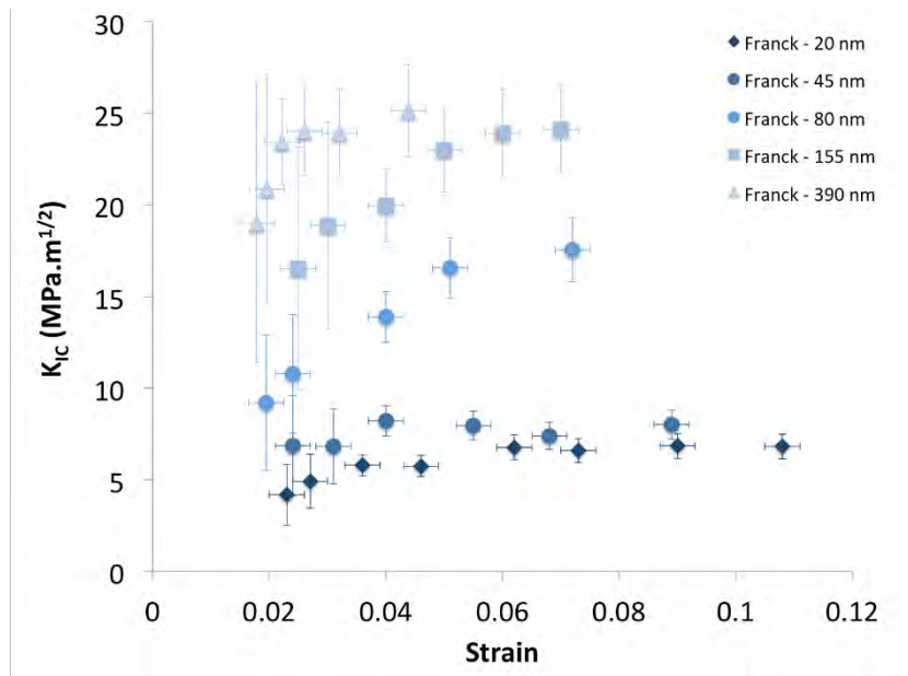
Figure 7.14 - K_{IC} as function of strain using Franck model for each thickness.
