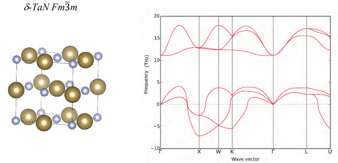
Figure A.2 - The phonon dispersion curves of \delta - TaN ( Fm\bar{3}m symmetry).
