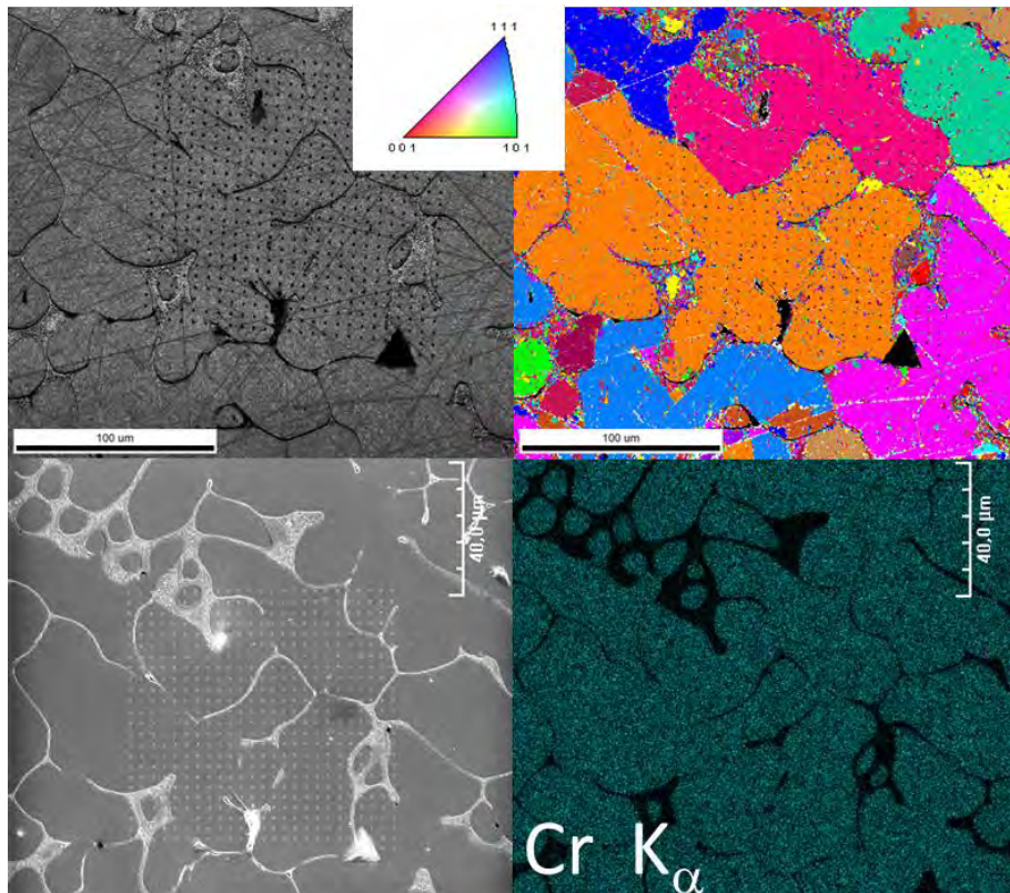
Figure 4.2 - SEM microstructure of as-cast CoCrCuFeNi , EDS mapping of Cr element and EBSD analysis at the same location. Indents from nanoindentation mapping are visible.
