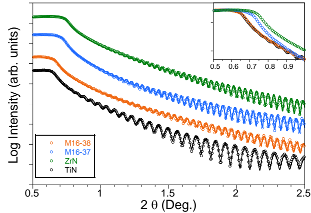
Figure 2.6: XRR scans (symbols) and best-fit curves (solid lines) from Ti_{1-x}Zr_xN_y films on MgO(001) substrate. The insert is a magnification around the critical angle.
