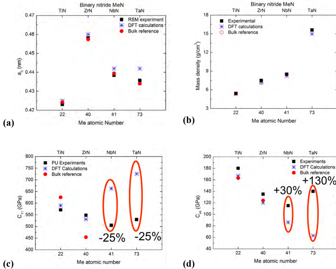
Figure 1.1 – Initial comparison between experimental and computational DFT of defect-free TiN , ZrN , NbN and TaN epitaxial films (a) Lattice parameter from XRD, (b) mass density from XRR, (c) c_{11} elastic constant from PLU, (d) c_{44} elastic constant from BLS.
