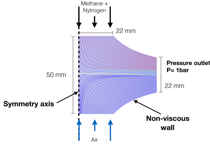
Figure 4.8 – Computational domain. The central axis is considered as symmetry axis and treated as a non viscous wall. The boundary walls of the domain are non-viscous and shaped like the streamlines of potential counter flow.
