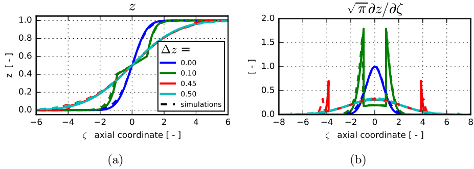
Figure 4.18 – Thickening operation with sensor with fixed value of F = 10 and different values of sensor size \Delta z . Comparison for the mixture fraction (a) and mixture fraction gradient (b) profiles. Continuous lines represent the analytical solutions, dashed line represent results from simulation in the Howarth-Dorodnitsyn axial coordinate.
