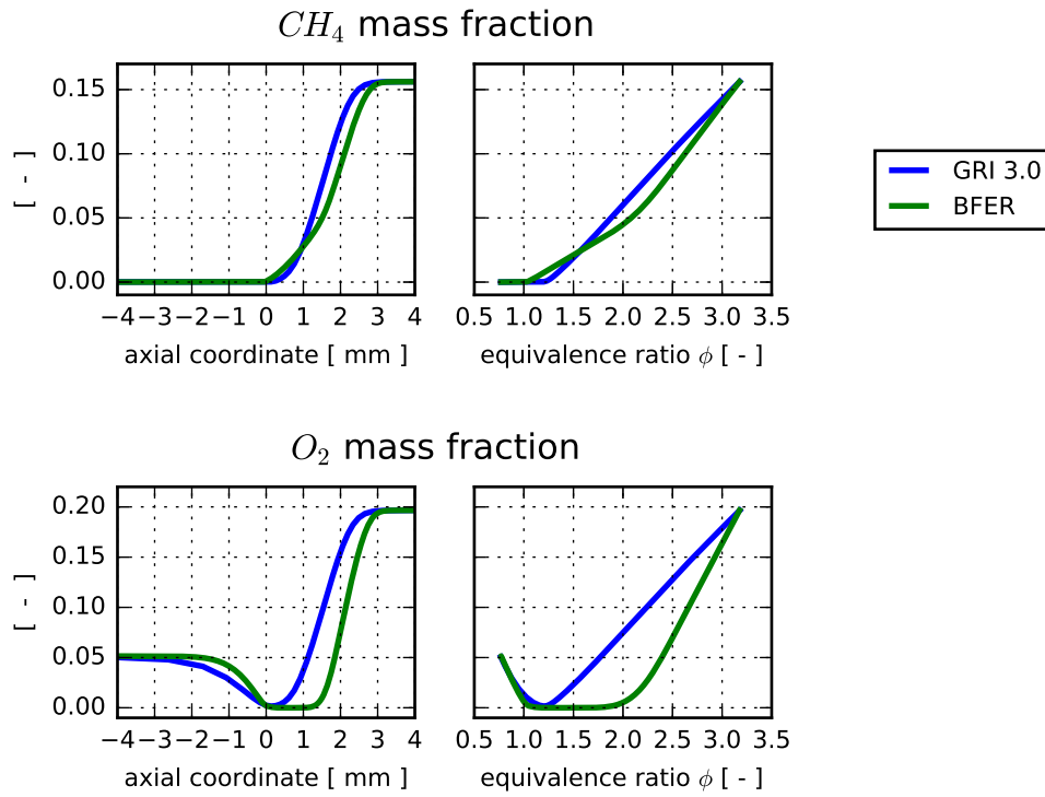
Figure A.8 – Comparison BFER mechanism with the detailed GRI 3.0 mechanism. Mass fraction profiles of CH_4 and O_2 over the axial coordinate and the equivalence ratio \phi .
