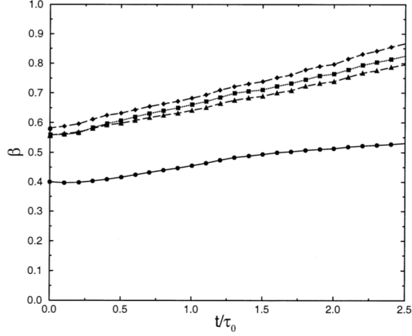
Figure 3.2 – Time evolution of dynamic parameter \beta . A-dimensional time as in figure 3.1. • F = 6.6 ; ■ F = 4.0 ; ◆ F = 2.8 \gamma = 2 ; ▲ F = 2.8 - \gamma = 3 (Charlette et al., 2002b).
