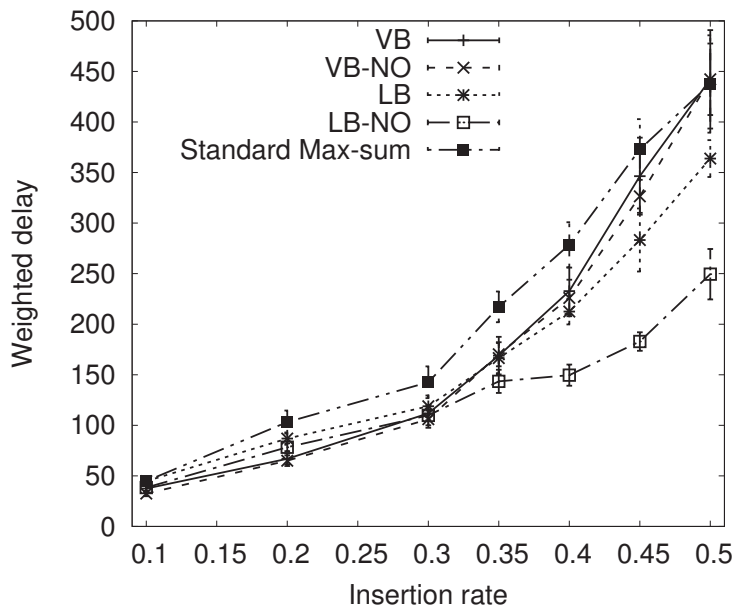
FIGURE 5.10: Average overall weighted delay.
