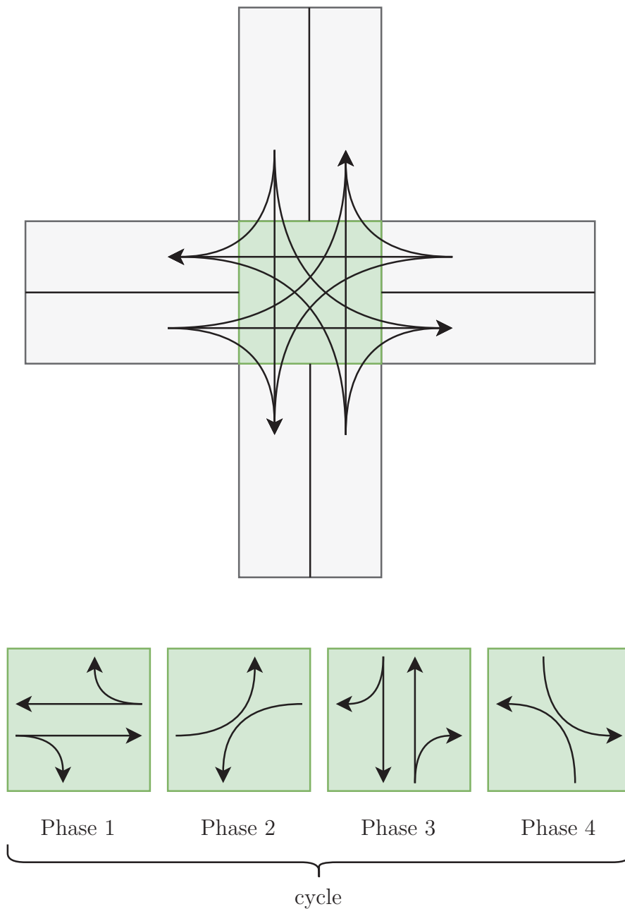
FIGURE 2.3: An intersection between two roads with 2 lanes each. 12 currents exist to cross this intersection. These currents can be decomposed into 4 groups of compatible currents (other cuttings are possible). The periods during which green and yellow are assigned to each of these groups of currents are the different phases forming the cycle.
