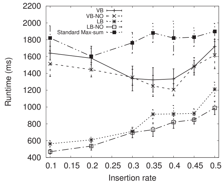
FIGURE 5.11: Average runtime when successful.
