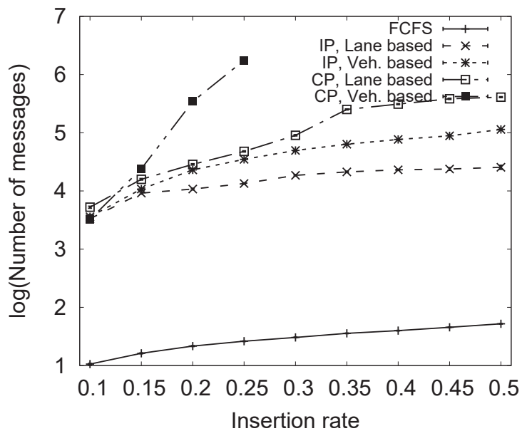
FIGURE 4.12: Average communication overhead at each iteration.
