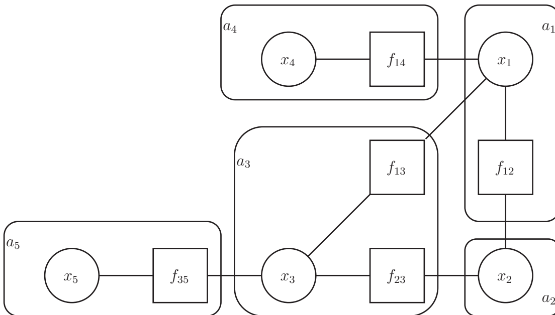
FIGURE 3.3: A factor graph describing the problem represented in Figure 3.1. A function node f_{ij} represents the constraint between x_i and x_j and is either controlled by a_i or a_j ,
