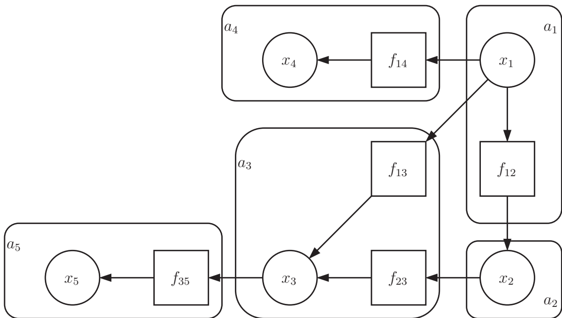
FIGURE 3.4: A directed factor graph used in Max-Sum_AD_VP describing the problem represented in Figure 3.1. Nodes are ordered using their index.
