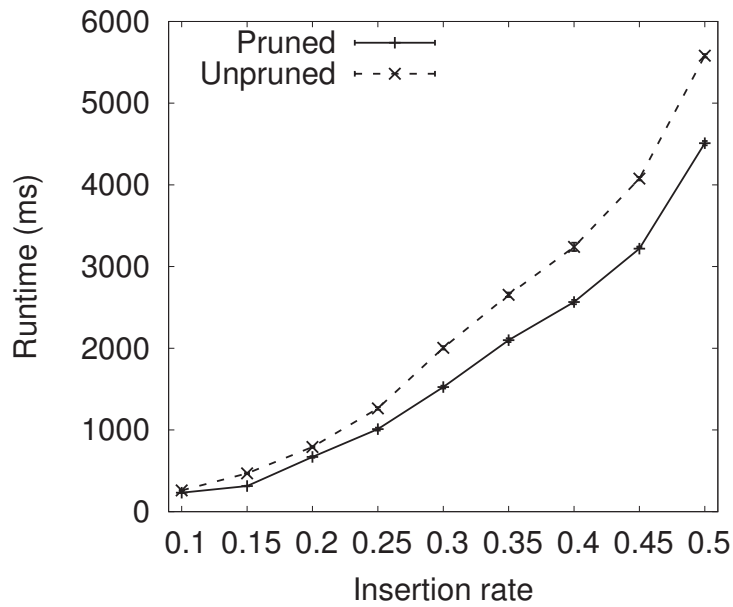
FIGURE 4.15: Average computational time comparison between the pruned and the standard version.
