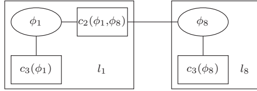
FIGURE 4.10: Lane-based factor graph for the scenario presented in Figure 4.1. Only two lanes have vehicles approaching the intersection so there are only two agents ( l_1 and l_8 ). Each agent holds an array variable node, \phi_1 contains \varphi_1 and \varphi_2 , \phi_8 contains \varphi_3 . There are 2 waiting time factor nodes ( c_3(\phi_1) and c_3(\phi_8) ), and 1 conflict factor node ( c_2(\phi_1, \phi_8) ).
