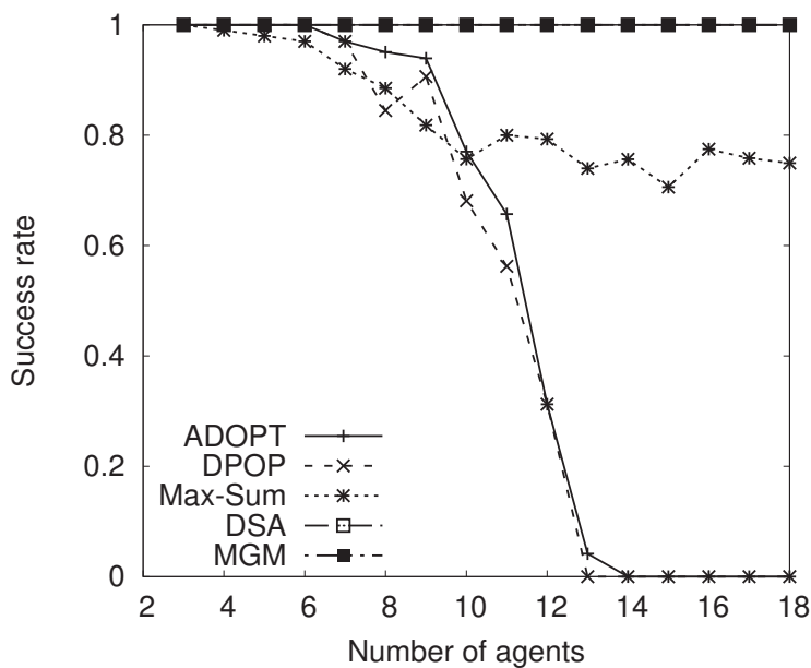
FIGURE 4.2: Average success rate of each algorithm.
