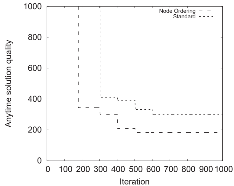
FIGURE 5.12: Anytime cost of ordered and standard versions of Max-sum_AD_VP running on the lane-based approach.
