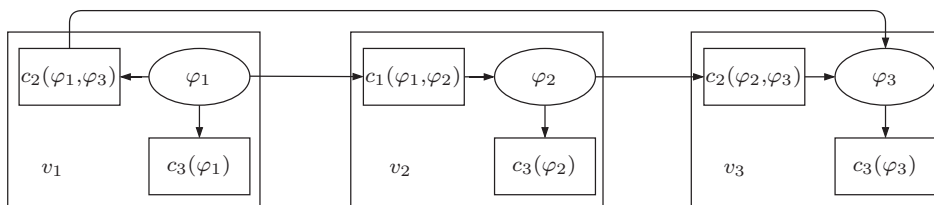
FIGURE 5.5: Vehicle-based directed factor graph for the scenario presented in Figure 5.2. There are 3 agents ( v_1, v_2, v_3 ), each holds an admission time as a variable node ( \varphi_1, \varphi_2, \varphi_3 ), 1 anteriority factor node c_1(\varphi_1, \varphi_2) , 2 conflict factor nodes ( c_2(\varphi_1, \varphi_3) and c_2(\varphi_2, \varphi_3) ), and 3 waiting time factor nodes ( c_3(\varphi_1) , c_3(\varphi_2) , and c_3(\varphi_3) ).
