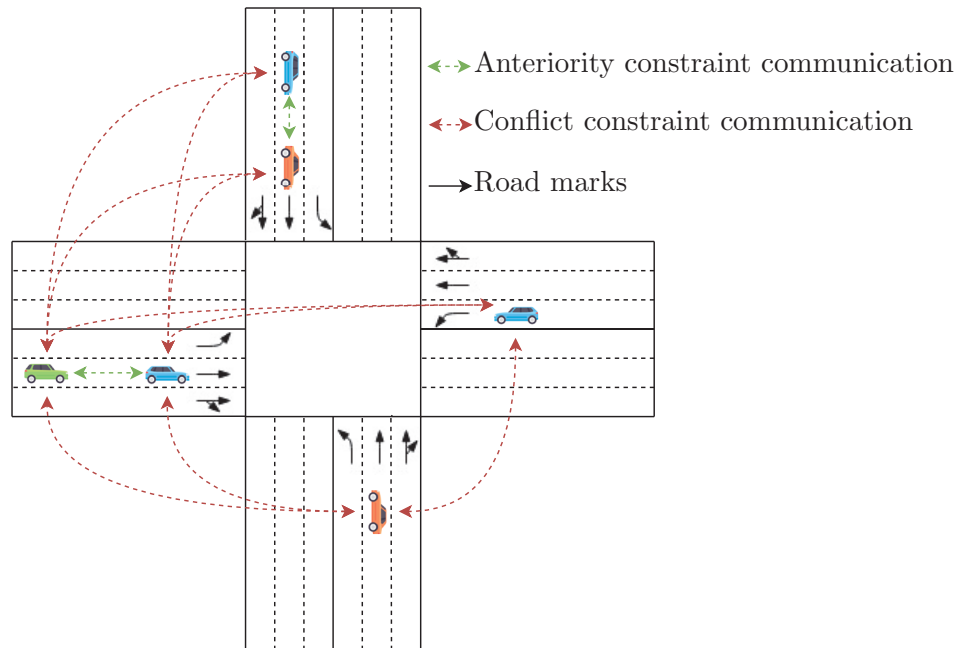
FIGURE 4.17: Communication range required for vehicle-based approach. Two vehicles need to be able to communicate with each other if they are constrained (i.e. either they are on the same lane, or they have conflicting trajectories). Therefore, the green vehicle on the western side has to communicate with the blue one on the north side. Such problem leads to higher communication range required.
