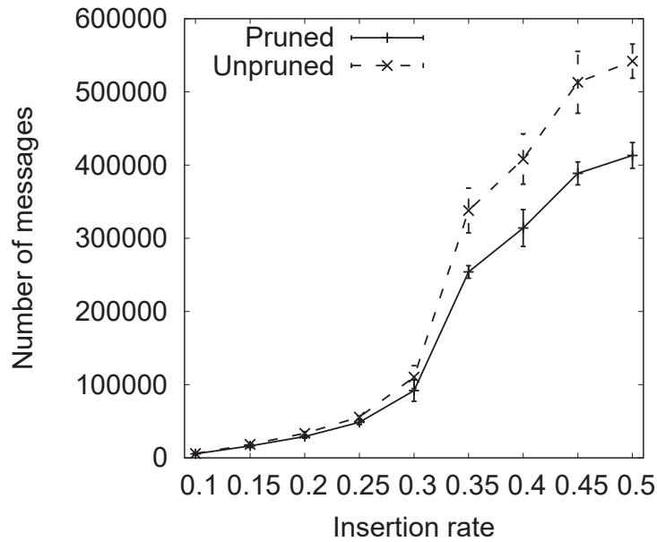
FIGURE 4.14: Average communication overhead comparison between the pruned and the standard version.
