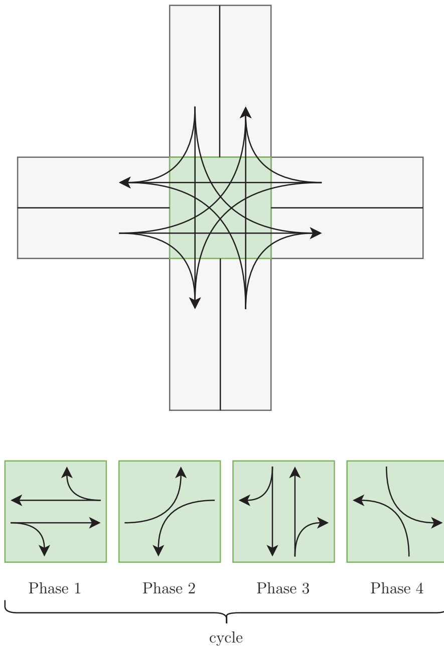
FIGURE 2.3: An intersection between two roads with 2 lanes each. 12 currents exist to cross this intersection. These currents can be decomposed into 4 groups of compatible currents (other cuttings are possible). The periods during which green and yellow are assigned to each of these groups of currents are the different phases forming the cycle.
