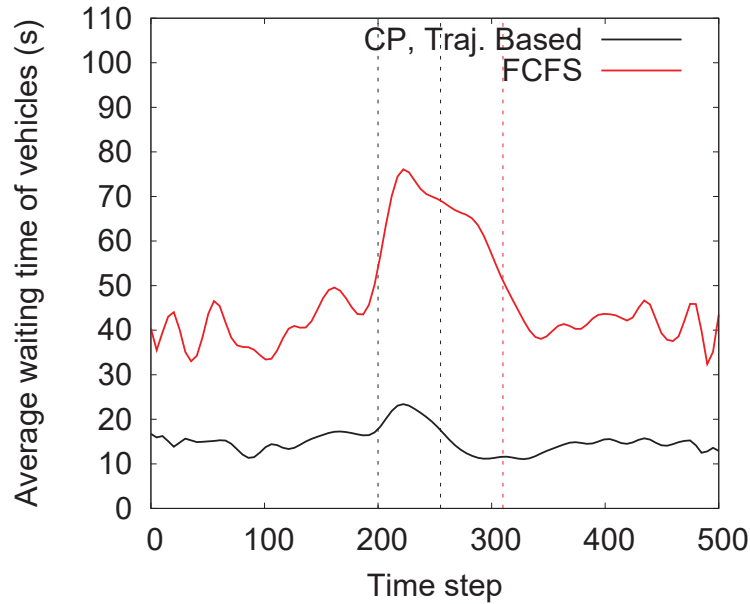
FIGURE 4.16: Average waiting time of vehicles at each time step. The emergency vehicle arrives at t = 200 . The CP stabilises at t \approx 250 while FCFS stabilises at t \approx 310 .
