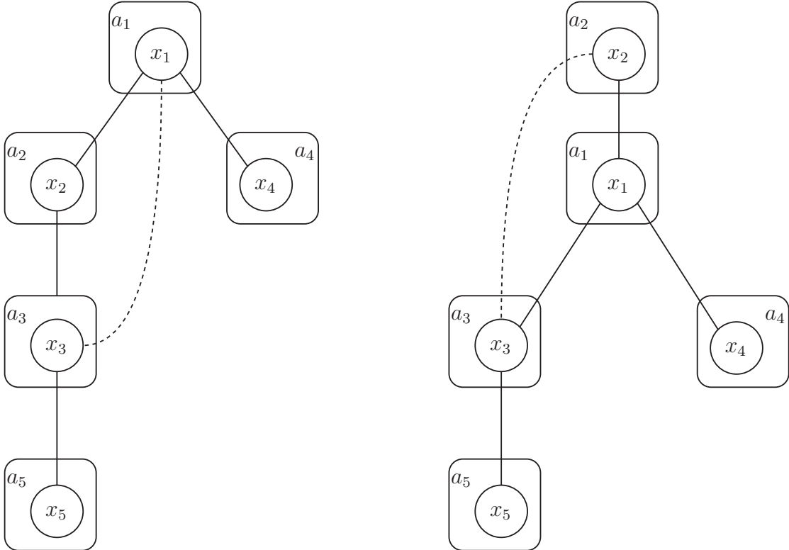
FIGURE 3.2: Two possible transformations of the Constraint Graph described in Figure 3.1 to a DFS tree. For example, on the left a_1 is the root node. Its descendants include every other nodes, while a_2 and a_4 are its direct childs. On the right is another possible way of transforming, using a_2 as the root node.
