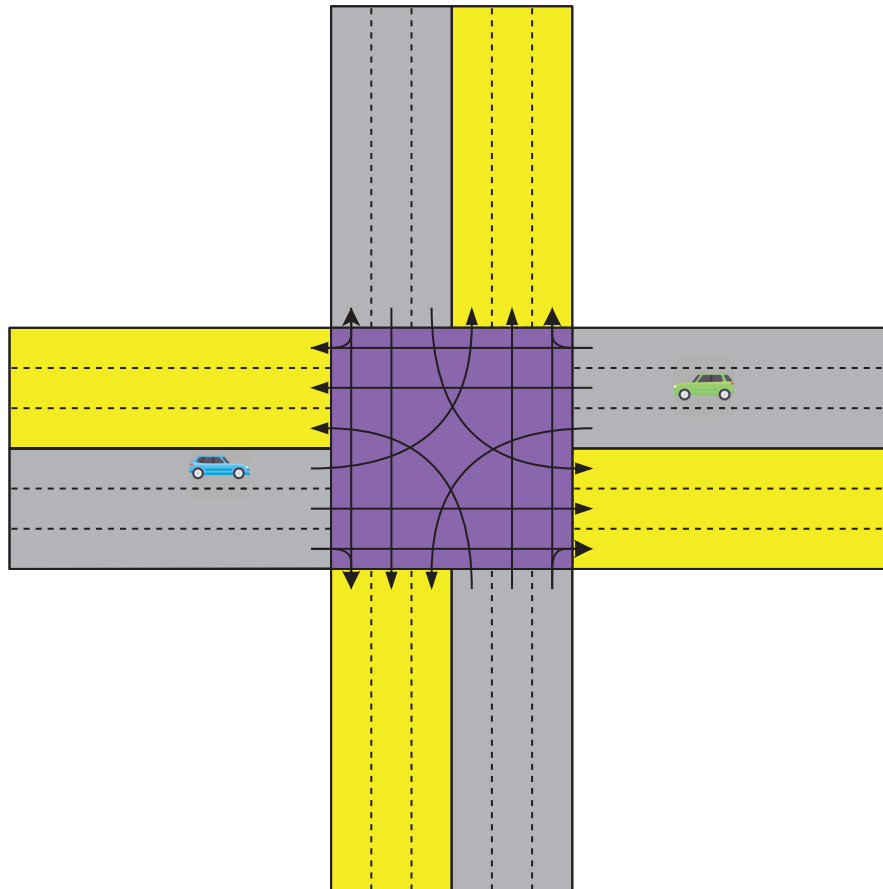
FIGURE 2.1: An intersection between two roads with 6 lanes each. Driving is on the right. The conflict zone is coloured in purple, the incoming lanes in gray and the outgoing lanes in yellow. The arrows represent the different possible vehicle streams. Thus the green vehicle or a vehicle on the same track can only go straight using the East-West current. The blue vehicle or a vehicle on the same track can only turn left using the West-North current.
