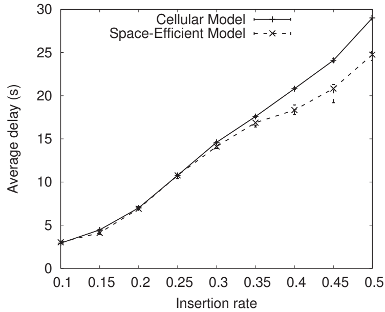
FIGURE 5.7: Performance of the space-efficient model compared to the cellular model.
