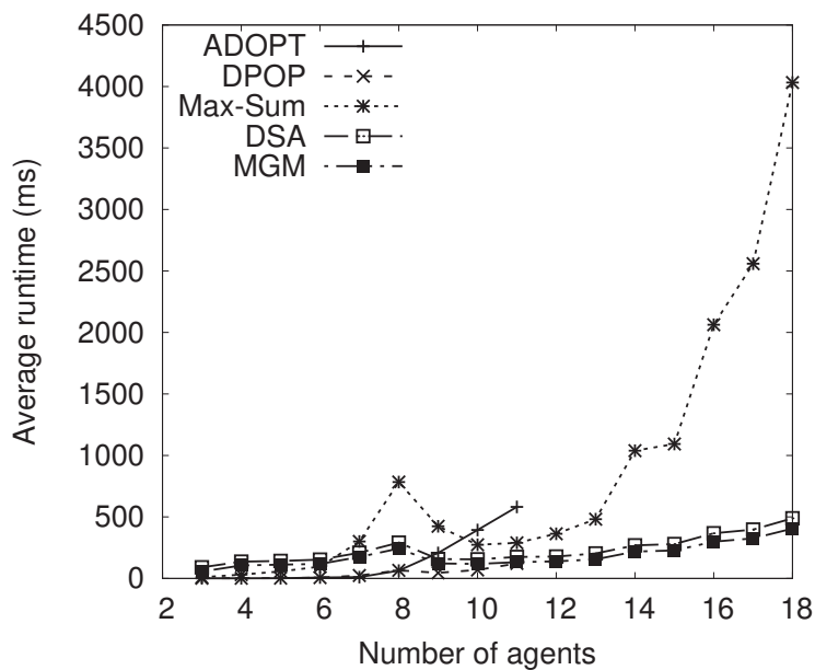
FIGURE 4.7: Average runtime of each algorithm. The results of ADOPT and DCOP from 12 agents are not shown due to the low success rate.
