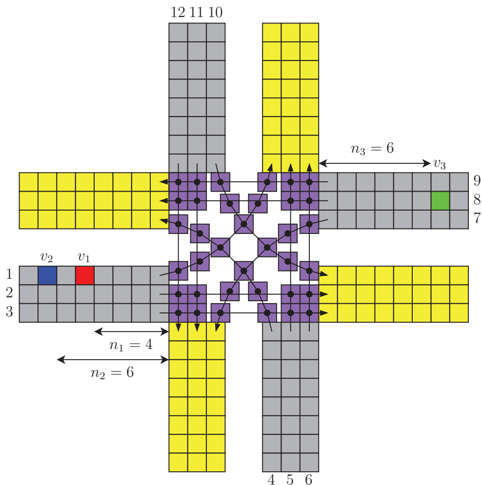
FIGURE 4.1: Intersection with 12 incoming lanes (in gray), 12 outgoing lanes (in yellow) and a conflict zone (in purple), all divided in cells. The incoming lanes are numbered from 1 to 12. The conflict zone is crossed by various trajectories. The cells belonging to several trajectories (every cell of the conflict zone in this case) are conflict spots. There are 3 vehicles v_1 (red rectangle), v_2 (blue rectangle) and v_3 (green rectangle). v_1 and v_2 are heading north, while v_3 is heading west.
