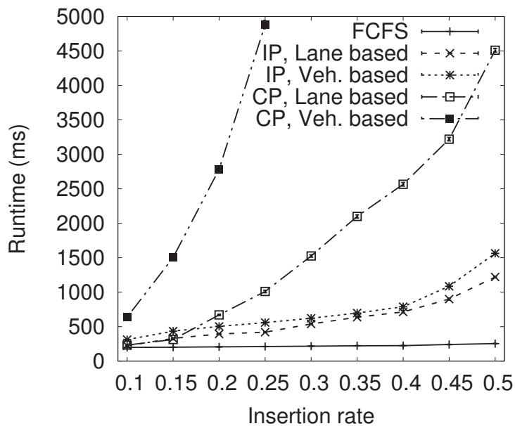
FIGURE 4.13: Average computational time at each iteration.
