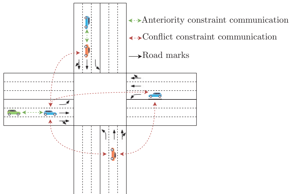
FIGURE 4.18: Communication range required for lane-based approach. Each lane is represented by a vehicle. To reduce communication range, the lane should be represented by the first vehicle on it. The communication is required between lane agents to solve conflicting trajectories. Other vehicles only need to communicate with their lane agent. The range required is therefore lower.
