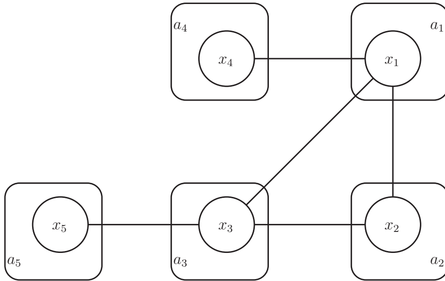
FIGURE 3.1: Example of a constraint graph representing five variables x_1 to x_5 , each controlled by one agent, a_1 to a_5 respectively. A link between two variables represents a constraint between them.
