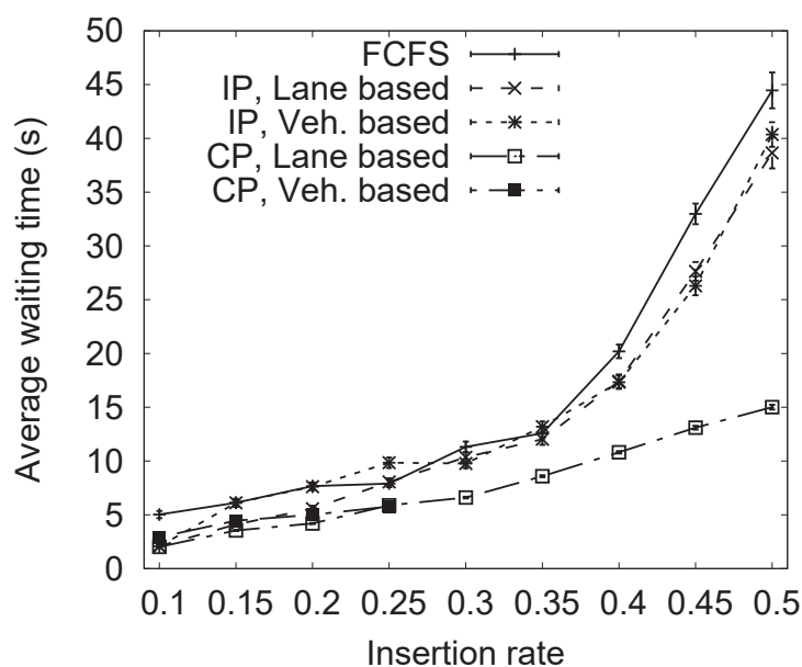
FIGURE 4.11: Average waiting time of vehicles.
