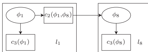
FIGURE 5.6: Lane-based directed factor graph for the scenario presented in Figure 5.2. Only two lanes have vehicles approaching the intersection so there are only two agents ( l_1 and l_8 ). Each agent holds an array variable node, \phi_1 contains \varphi_1 and \varphi_2 , \phi_8 contains \varphi_3 . There are 2 waiting time factor nodes ( c_3(\phi_1) and c_3(\phi_8) ), and 1 conflict factor node ( c_2(\phi_1, \phi_8) ).
