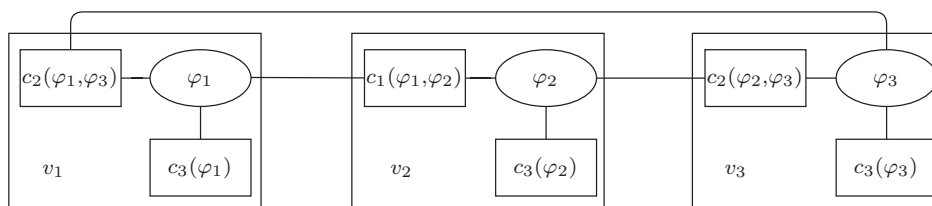
FIGURE 4.9: Vehicle-based factor graph for the scenario presented in Figure 4.1. There are 3 agents ( v_1, v_2, v_3 ), each holds an admission time as a variable node ( \varphi_1, \varphi_2, \varphi_3 ), 1 anteriority factor node c_1(\varphi_1, \varphi_2) , 2 conflict factor nodes ( c_2(\varphi_1, \varphi_3) and c_2(\varphi_2, \varphi_3) ), and 3 waiting time factor nodes ( c_3(\varphi_1) , c_3(\varphi_2) , and c_3(\varphi_3) ).
