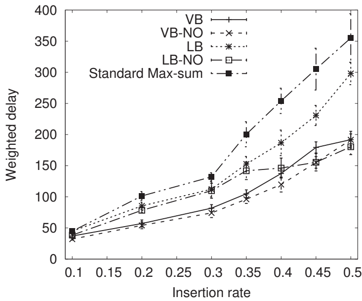
FIGURE 5.9: Average solution quality when successful.
