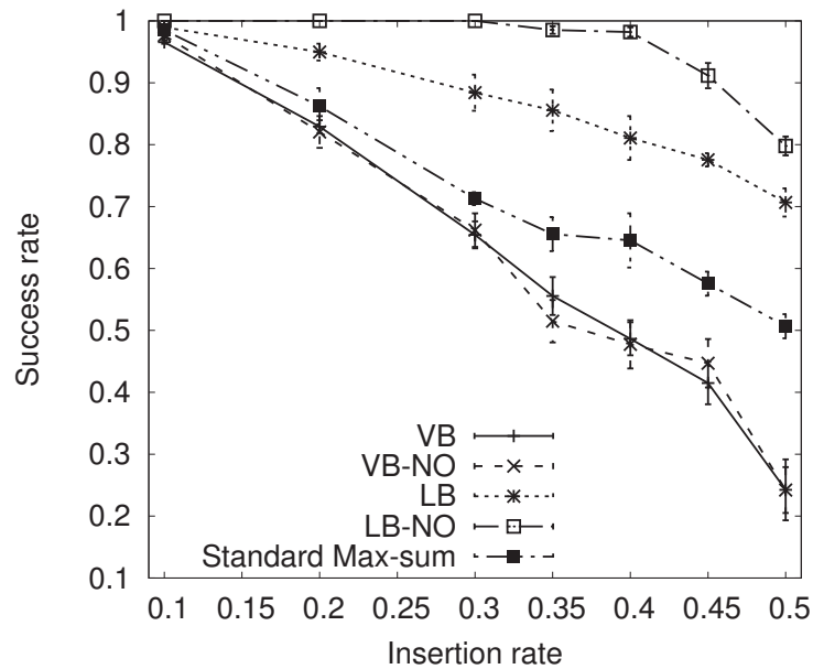
FIGURE 5.8: Success rates of each approach on a weighted delay problem.
