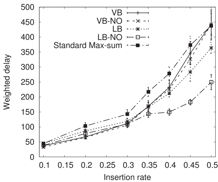
FIGURE 5.10: Average overall weighted delay.
