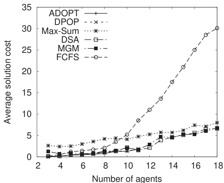
FIGURE 4.3: Average solution quality of each algorithm. The results of ADOPT and DCOP from 12 agents are not shown due to their low success rate.
