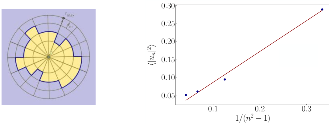
FIGURE 4.13 – Left: Scheme of the polar discretization (r, \theta) applied to a Lo domain and determination of the Lo-Ld boundary as a function r(\theta) . Courtesy of Nelly Coulonges. Right: Power spectrum of the Lo-Ld boundary in a DPPC-DIPC-chol mixture from which the line tension \lambda is extracted. The values of the y -axis must be divided by 2\pi^2 .
