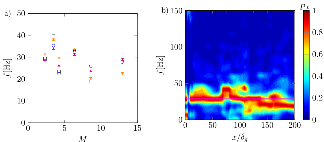
Fig. 3.7 – (Color online) a) Most amplified frequency of the interface height signal as a function of the dynamic pressure ratio for all cases of table 3.2. \square : experimental results (Matas et al., 2011), \triangle : linear stability analysis results, * : simulation results with n = 2 , \circ : simulation results with n = 8 . b) Spectrogram of the interface height signal for case A1, with n = 8 . The horizontal magenta line represents the predicted wave frequency.
