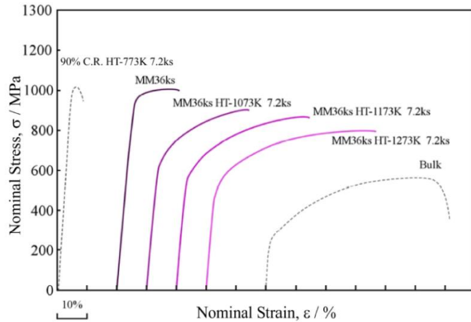
Fig. 2.18 Nominal stress-strain curves of the HRS compacts with various post heat treatments in comparison with the experimental result of the 90% cold rolled and heat treated bulk material (Fujiwara et al., 2010).
