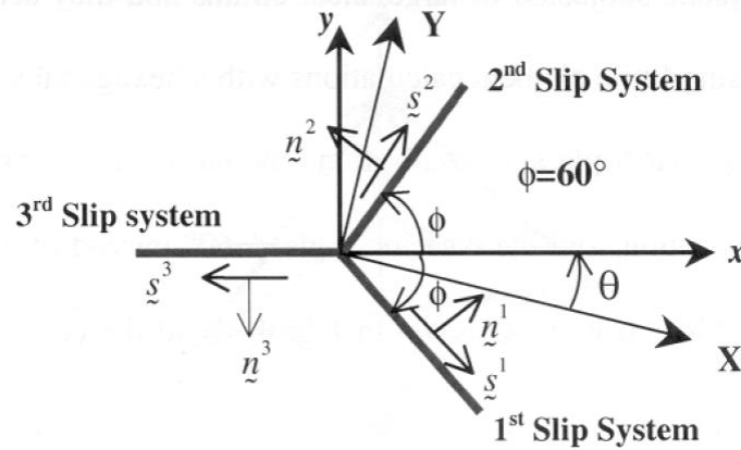
Fig. 6.1 Slip geometry of the planar triple slip model where the angle \theta completely specifies the orientation of the grain (Morrissey, 2001; Goh, 2002).
