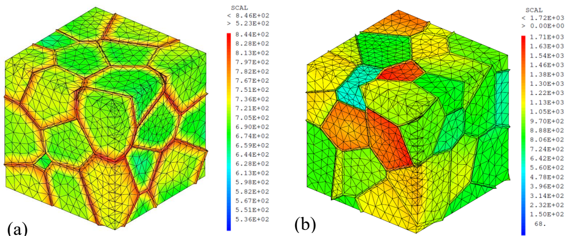
Fig. 6.11 Effective shear stress distribution for (a) HS CP-Ti when \Gamma = 24.0\% and (b) HS Ti-6Al-4V when \Gamma = 12.7\% .
