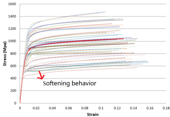
Fig. B.4 Illustration of intergranular heterogeneity based on the volume averaged responses of 50 equivalent grains for lamellar \alpha+\beta colonies.
