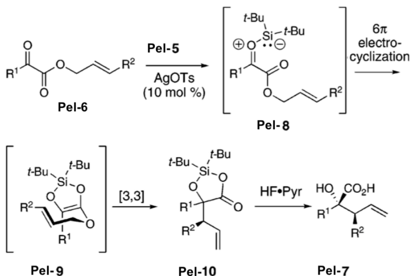
Scheme 13: Proposed mechanism 38
