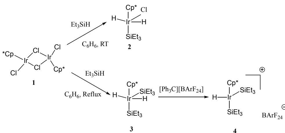
Scheme 21: Synthesis of 2, 3, 4
