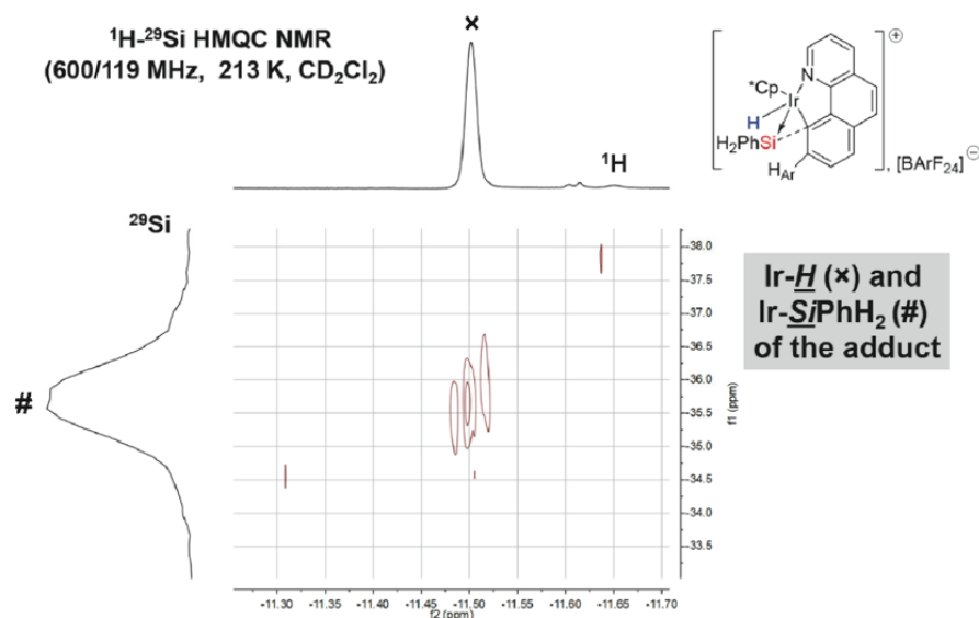
Figure 11: cross-peak correlation with a ^{29}\text{Si} of Ir-H of [2c][\text{BARF}_{24}]
