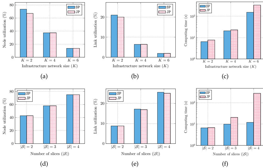
Figure 5.2: Performance of JP and SP as function of the fat-tree size ( K ) and of the number of slices ( |S| ), in terms of (a, d) utilization of infrastructure nodes, (b, e) utilization of infrastructure link, and (c, f) computing time.
