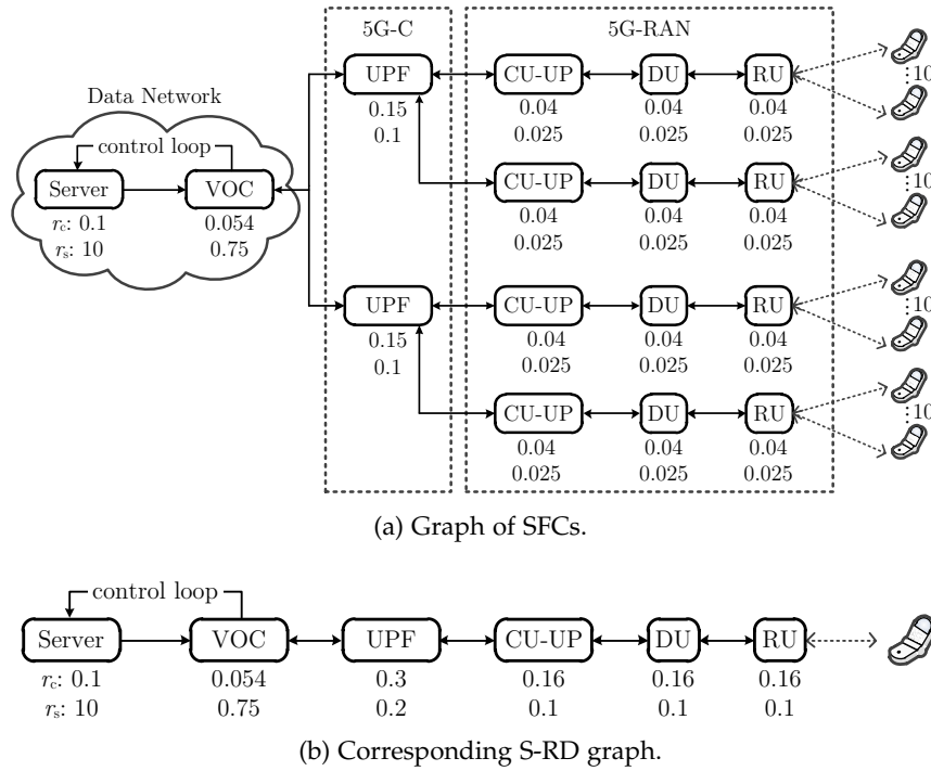
Figure 4.4: Virtual graph and the required computing (in CPUs) and memory (in GBytes) resources for the deployment of SFCs and slice dedicated to an adaptive wireless video streaming service.
