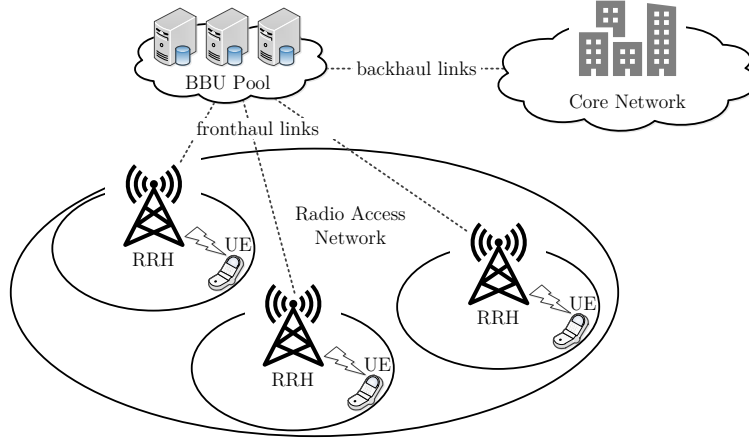
Figure 4.3: General architecture of C-RAN
