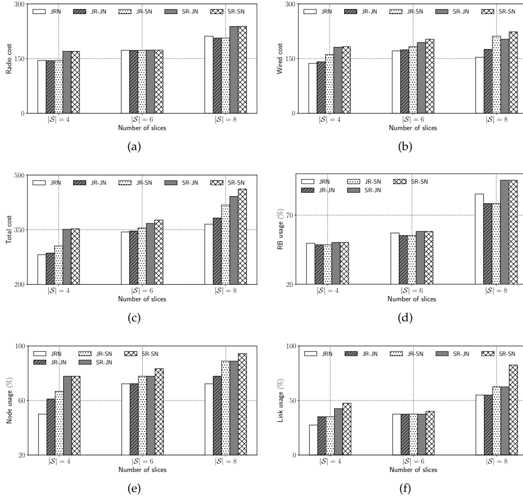
Figure 6.3: Performance comparison of 4 variants in terms of (a) radio cost, (b) wired cost, (c) total provisioning cost, utilization of (d) RBs, (e) infrastructure nodes, and (f) infrastructure links.
