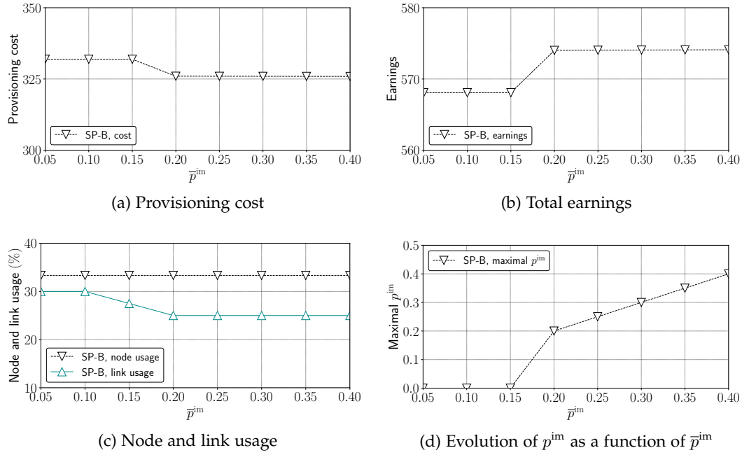
Figure 7.3: Performance of the SP-B approach on single slice provisioning problem with different values of \bar{p}^{im} , in terms of (a) provisioning costs, (b) total earnings, (c) node and link utilization, and (d) maximal impact probability p^{im} .
