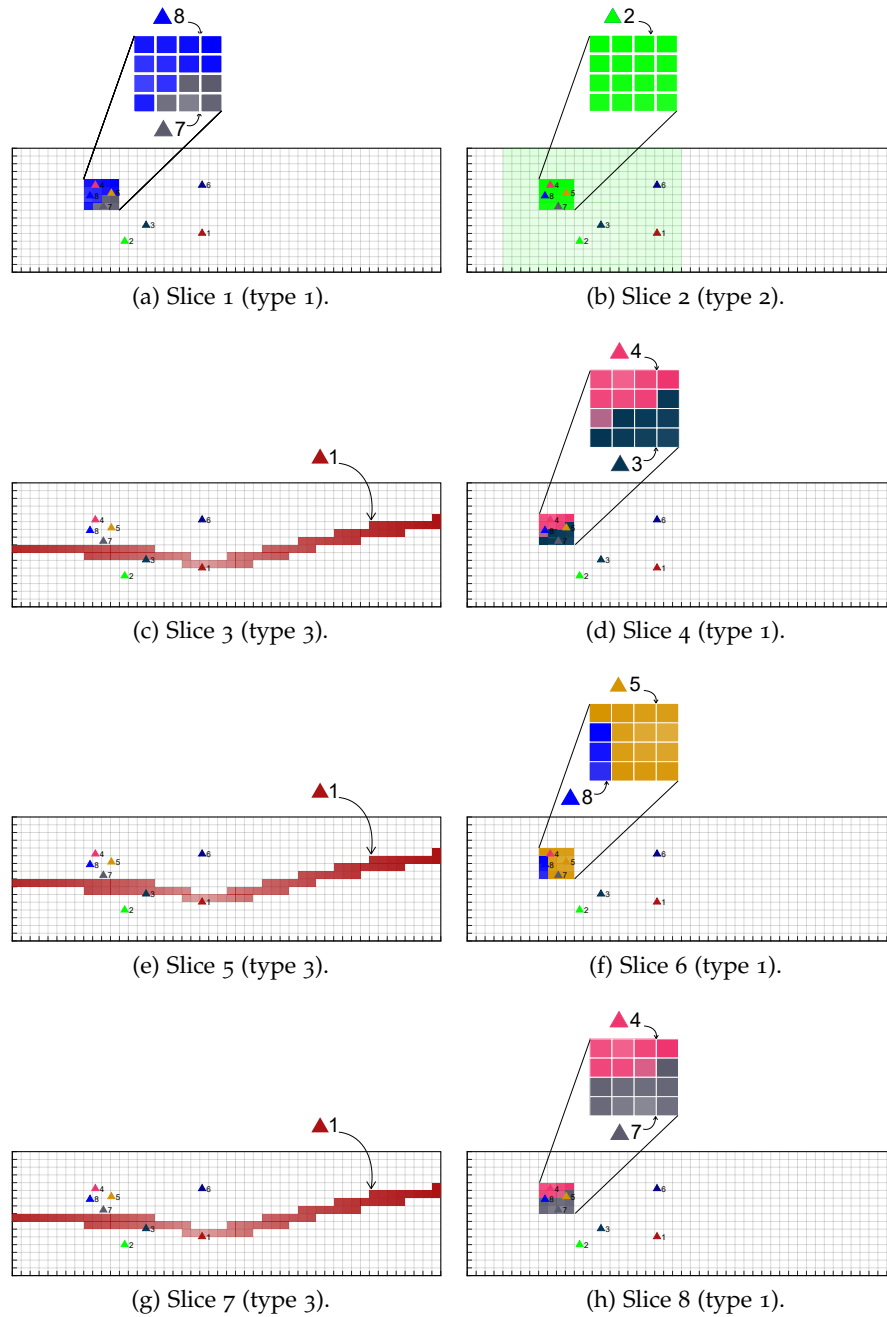
Figure 6.7: Usage of RBs by each slice using JRN method. RRHs are represented by triangles with different colors. Subareas (small squares) of each provisioned slice are filled by the same color of the RRH that provisions RBs for that slice. The color density reflects the amount of provisioned RBs (the darker, the more RBs).
