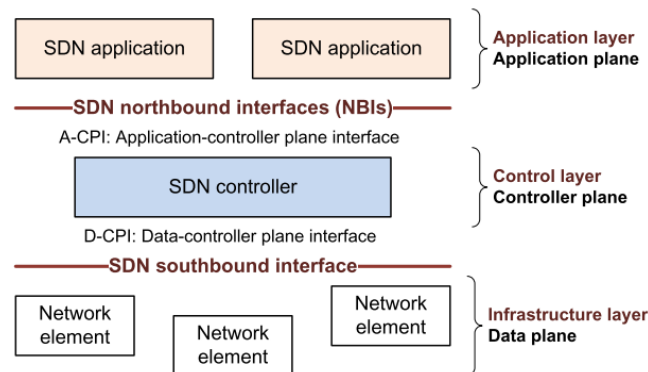
Figure 2.4: Fundamental components of SDN [ONF, 2014].
