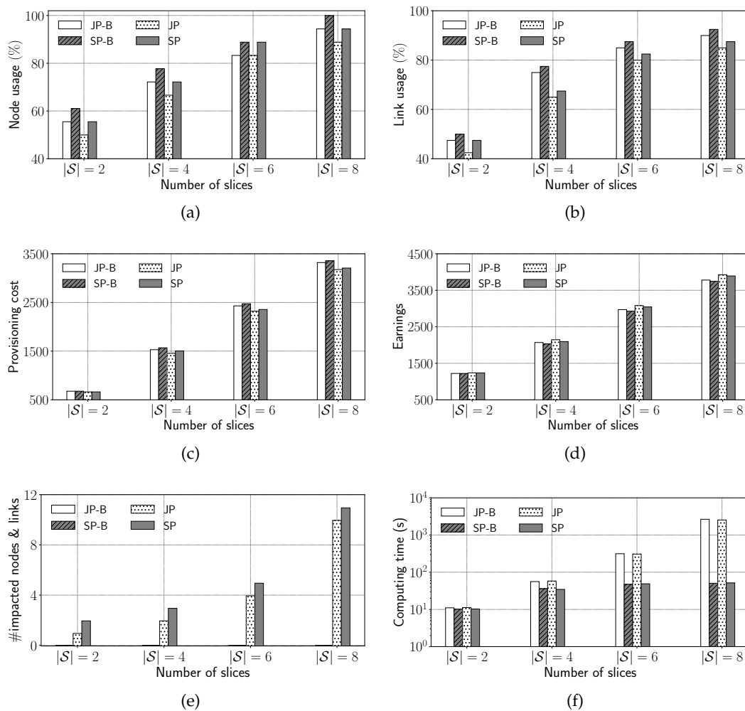
Figure 7.5: Performance comparison of 4 variants in terms of (a) utilization of infrastructure nodes, (b) utilization of infrastructure links, (c) provisioning costs, (d) total earnings, (e) number of impacted nodes and links, and (f) computing time.
