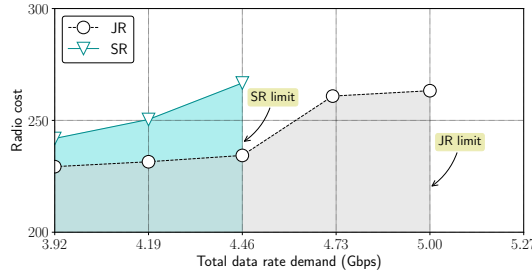
Figure 6.5: Maximum supported data rate associated to the SR and JR provisioning approaches when 3 slices of type 1, 2, and 3 have to be deployed.
