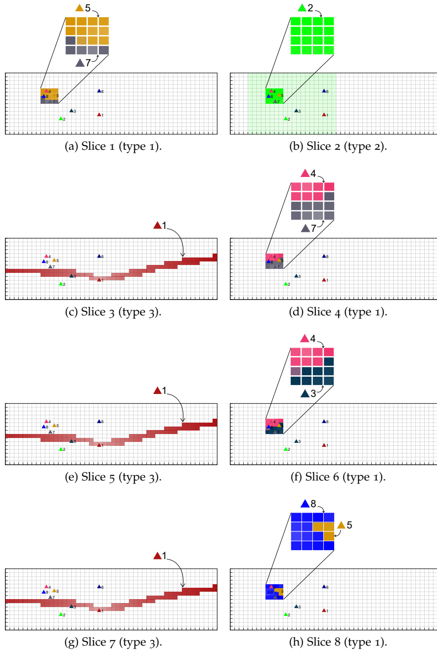
Figure 6.8: Usage of RBs by each slice using JR-SN method. RRHs are represented by triangles with different colors. Subareas (small squares) of each provisioned slice are filled by the same color of the RRH that provisions RBs for that slice. The color density reflects the amount of provisioned RBs.
