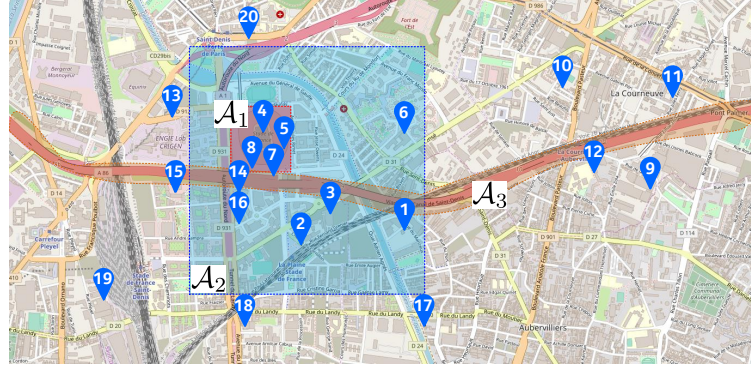
Figure 6.1: The considered metropolitan area including the Stade de France (covered by the red rectangle representing \mathcal{A}_1 ), its surrounding (blue rectangle representing \mathcal{A}_2 ), and part of the A86 highway (orange shape representing \mathcal{A}_3 ); Blue markers show the location of RRH nodes of Orange.
