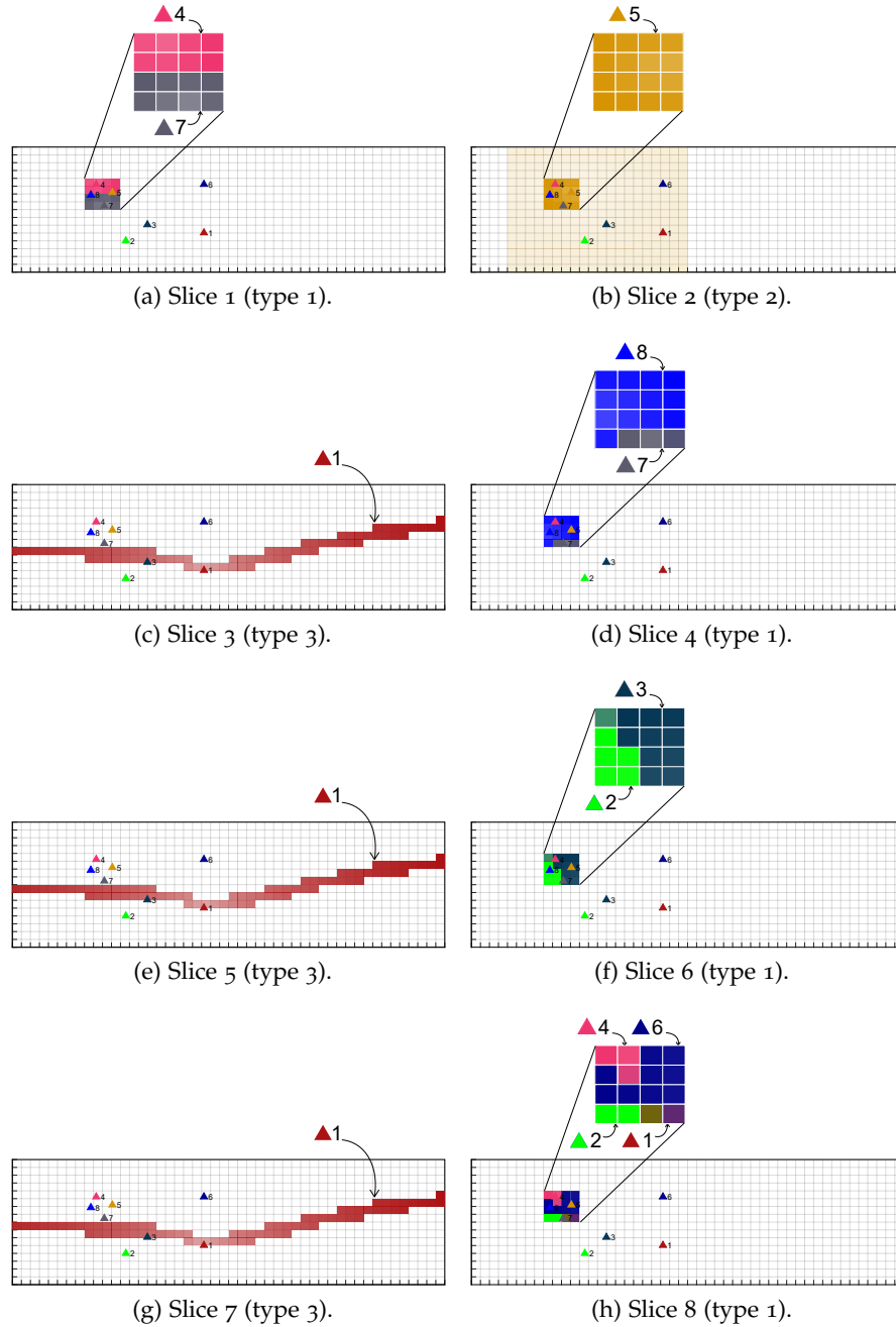
Figure 6.9: Usage of RBs by each slice using SR-SN method. RRHs are represented by triangles with different colors. Subareas (small squares) of each provisioned slice are filled by the same color of the RRH that provisions RBs for that slice. The color density reflects the amount of provisioned RBs.
