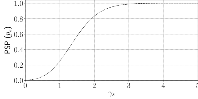
Figure 7.2: Evolution of p_s as function of \gamma_s .
