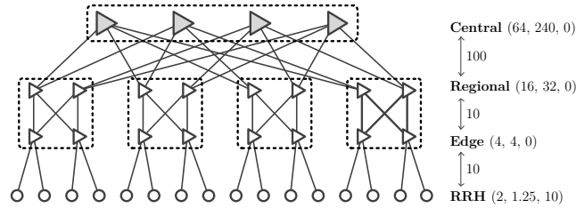
Figure 5.1: Description of the infrastructure network. Nodes provide a given amount of computing, memory, and possibly wireless resources ( a_c, a_m, a_w ) measured in number of used CPUs, Gbytes, and Gbps, respectively. Links are assigned with a given amount of bandwidth ( a_b ) measured in Gbps.
