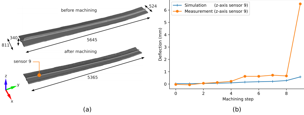
Figure 1.7: Example of distortion in a cruciform. (a) Geometry before and after machining. (b) Simulation vs measurements results. Adapted from [19].
