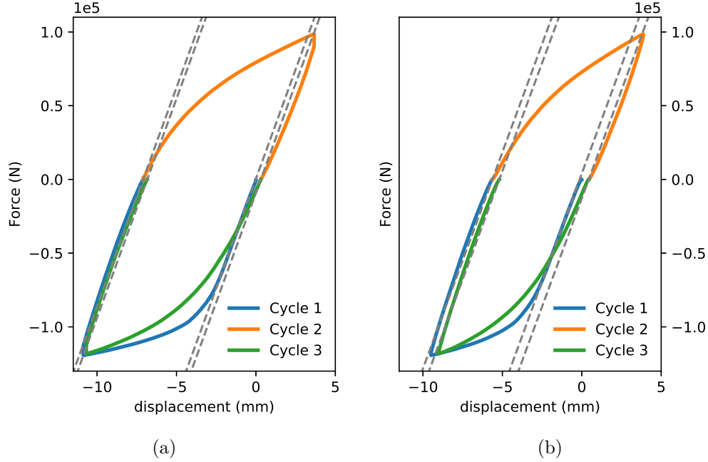
Figure 3.9: Testing the linear unloading hypothesis. Force versus displacement diagram for the rectangular rolled plate (specimen L2). Experimental curves (solid lines) vs linear unloading path (dashed lines). (a) At midspan L = 100 mm and (b) At the section where the load is applied L = 70 mm (see Figure 2.5a).
