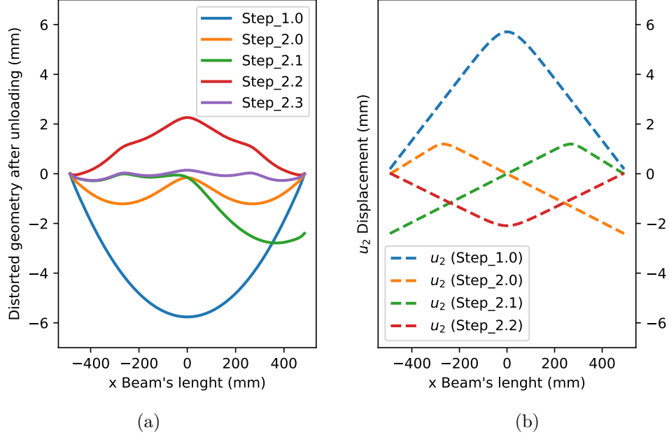
Figure 5.8: Distortion evolution during reshaping (simulation results). (a) Distorted geometry after unloading. (b) Imposed vertical displacement u_2 for each reshaping step.
