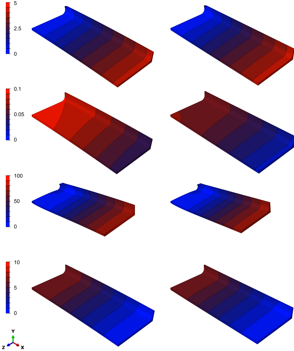
Figure 4.8: First 8 snapshots of the displacement field u(x; \mu) . From left to right \delta_0 = [-15, 0] . From top to bottom the pair (y_s, r_e) are (5, 100) , (5, 485) , (30, 100) and (30, 485) , respectively.
