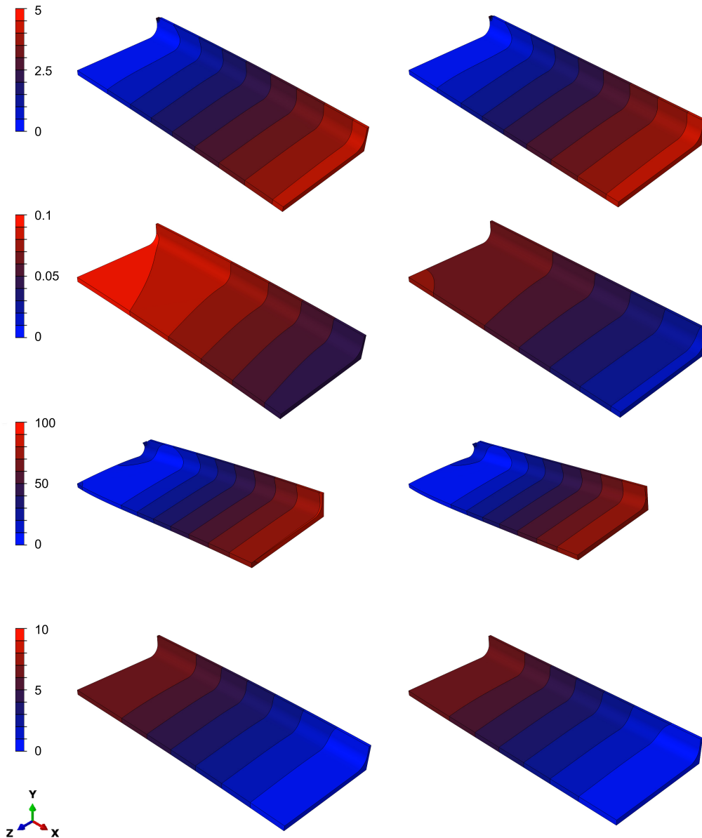
Figure 4.8: First 8 snapshots of the displacement field \mathbf{u}(\mathbf{x}; \boldsymbol{\mu}) . From left to right \delta_0 = [-15, 0] . From top to bottom the pair (y_s, r_e) are (5, 100) , (5, 485) , (30, 100) and (30, 485) , respectively.
