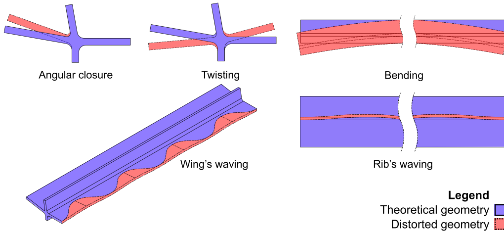
Figure 1.3: Principal types of distortion after machining in a simplified version of the Airbus' A320 cruciform beam. Adapted from [65].
