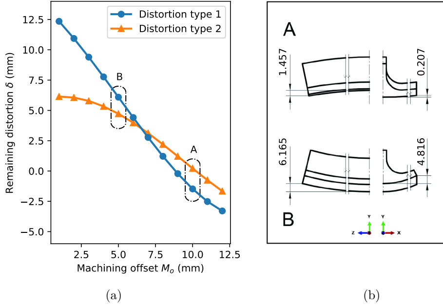
Figure 3.5: T shaped beam model. (a) Distortion after machining as a function of machining offset M_o . (b) Distorted shape for case A ( M_o = 10 mm) and case B ( M_o = 5 mm).
