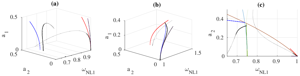
Figure 11.4.6: Backbone curves of the system, (a): coefficients are chosen as Eq. (11.3.6) and \omega_1 = 1 , \omega_2 = 1.5 ( \sigma < 0 ), (b): coefficients are chosen as Eq. (11.4.13) and the \omega_1 = 1 , \omega_2 = 2.5 ( \sigma > 0 ). (c): Top view of plot (a), with the brown curve is computed by Eq. (11.2.5a) with a_1 = 0 , the cyan curve is computed by \frac{1}{2}\omega_{NL2}^{s dof} , and the green curve presents the \frac{1}{2}\omega_{NL2}^{s dof} computed on the ROM with continuous computation tool. In the figure, the analytical results of the normal form with 1:2 internal resonance are given in blue ( p- mode) and red ( p+ mode), also the result of single NNM is in purple, and the results of the original system calculated by the Manlab are shown in black, with the unstable solution dotted.
