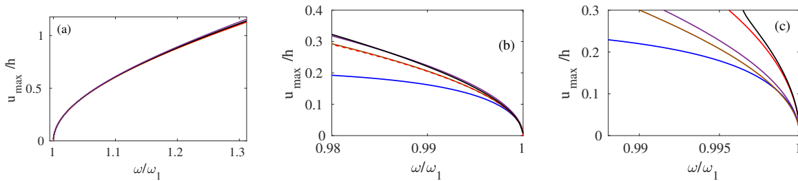
Figure 7.1.3: The backbone curves for (a) the straight beam, (b) the shallow arch, and (c) the non-shallow arch. reference solution with numerical continuation in black. Comparison of reduction methods with a single master coordinate, purple: ICE method, blue: QM-SMD, brown: QM-MD and red: DNF.
