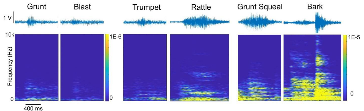
Figure 20. Six types of vocalizations recorded during the session. Top panel : Acoustic waveforms of averaged vocalizations for each recorded call type. Bottom panel : narrow band spectrograms of averaged vocalizations for each recorded call type. The spectrograms were generated in Matlab using the following parameters : 150ms window size, frequency range : 0-10kHz, frequency steps : 300. Grunt and Blast spectrogram scales range from 0 to 1E-6 \mu\text{V}/\sqrt{\text{Hz}} . The other vocalizations spectrogram scales range from 0 to 1E-5 \mu\text{V}/\sqrt{\text{Hz}} . Temporal scale of 400ms is common to all the panels. Amplitude scale of 1V is common to all the acoustic waveforms.
