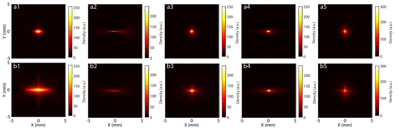
FIGURE 3.21: Simulated electron beam transverse shape at the (a1, b1) first imager, (a2, b2) “Chicanes”, (a3, b3) “UndIn”, (a4, b4) undulator entrance and (a5, b5) “UndOut”. Energy distribution from a_{0,initial}=1.75 , n_e = 4.56 \times 10^{18} and 1 % N_2 concentration (Figure 5.19) PIC simulation and initial electron beam characteristics \epsilon_{x,y,RMS}=1 mm.mrad, (a) \sigma'_{x,y,RMS}=1 mrad, Q_{176\pm 0.5\text{MeV}}=10.3 pC, (b) Q_{176\pm 0.5\text{MeV}}=1 pC, \sigma'_{y,RMS}=2 mrad, \sigma'_{x,RMS}=3.12 mrad.
