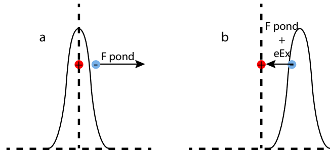
FIGURE 2.2: Ponderomotive force of a laser pulse on electrons inside plasma.
