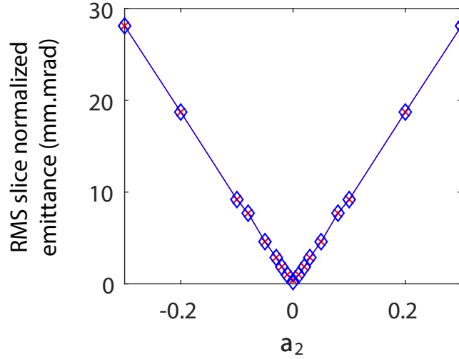
FIGURE 6.28: Simulated slice 176 \pm 0.1 MeV horizontal ( \times ) and vertical ( \diamond ) RMS normalized emittance of the electron beam at the undulator center versus QUAPEVA 2 a_2 skew term with the “slit-undulator” optics and the slit open to 3.2 mm. Simulation using a flat-top beam with \sigma'_{y,i,RMS} = 2 mrad and \sigma'_{x,i,RMS} = 3.12 mrad, \epsilon_{y,i,RMS}, \epsilon_{x,i,RMS} = 0.2 mm.mrad [178].
