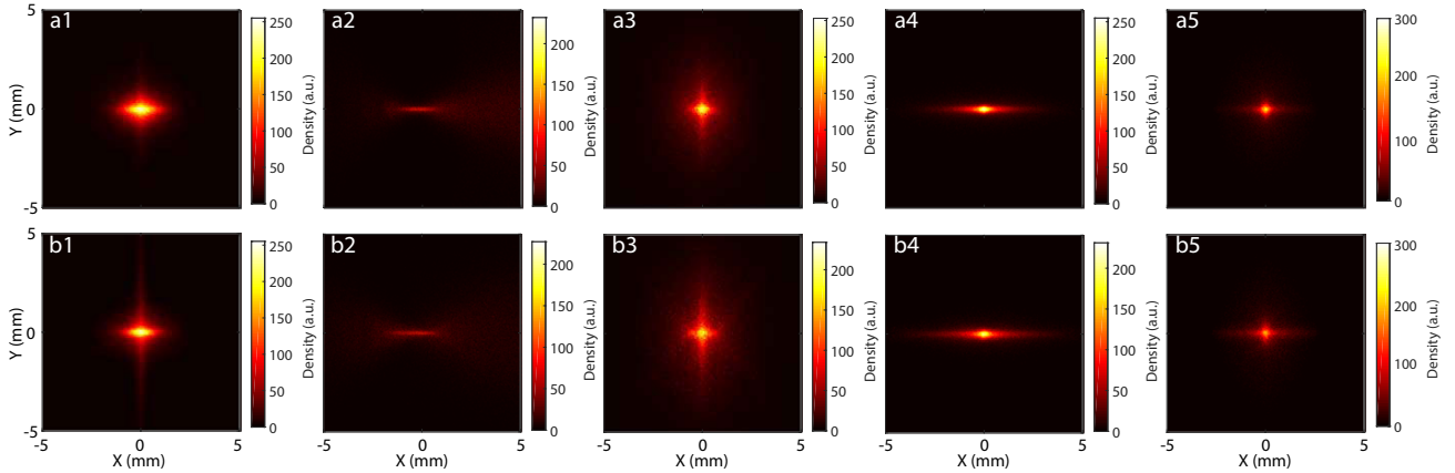
FIGURE 6.7: Simulated electron beam transverse shape at the (a1, b1) first imager, (a2, b2) “Chicane”, (a3, b3) “UndIn”, (a4, b4) undulator entrance and (a5, b5) “UndOut”. Energy distribution from a_{0,initial}=1.75 , n_e = 4.56 \times 10^{18} and (a) 1 %, (b) 2 % N_2 concentration (Figure 5.19) PIC simulation, Q_T = 100 pC.
