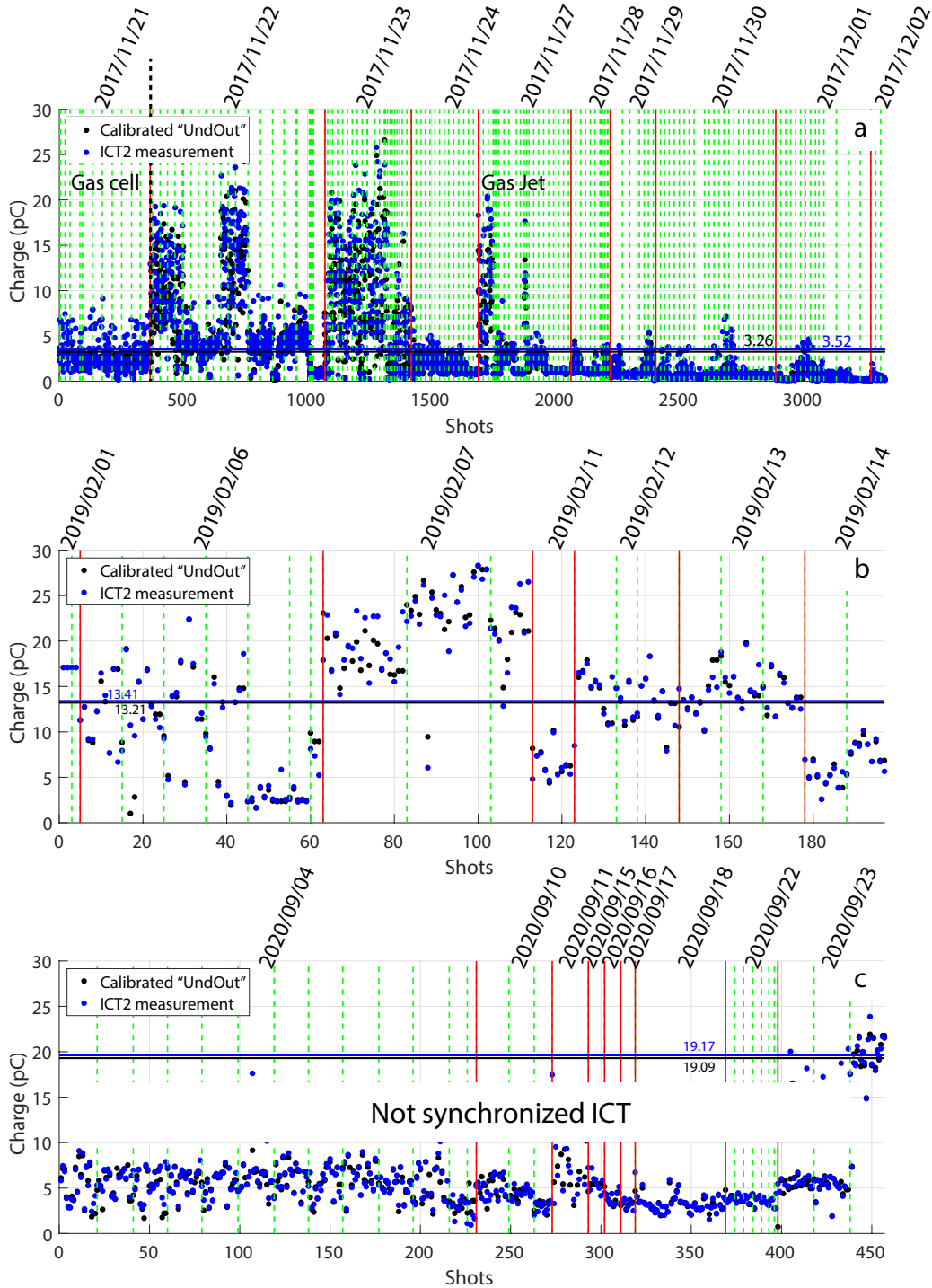
FIGURE 7.23: Measured total beam charge after the undulator on (blue) the ICT2 and (black) at the calibrated imager “UndOut” during RUN 4 (a), 6 (b) and 7 (c) in chronological order, separation by configuration (black dotted line), day (red line) and series (green line).
