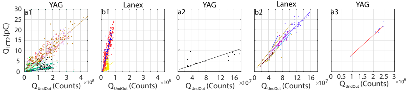
FIGURE 7.19: Charge measured after the undulator at the ICT2 versus imager “UndOut” total counts after image treatment and (line) linear fits for count/pC calibration with the (a) YAG and (b) Lanex screens. Run (a1, b1) 4, (a2, b2) 6 and (a3) 7 data each color representing a day. RUN 4 (a1, b1): 2017/11/21 (YAG black, Lanex yellow), 2017/11/22 (YAG pink, Lanex red), 2017/11/23 (YAG brown, Lanex blue), 2017/11/24 (YAG green), 2017/11/27 (YAG purple), 2017/11/28 (YAG yellow), 2017/11/29 (YAG crimson), 2017/11/30 (YAG light green), 2017/12/01 (YAG emerald), 2017/12/02 (YAG dark brown). RUN 6 (a2, b2): 2019/02/01 (Lanex blue), 2019/02/06 (YAG black, Lanex brown), 2019/02/07 (Lanex purple), 2019/02/11 (Lanex light brown), 2019/02/12 (Lanex cyan), 2019/02/13 (Lanex pink), 2019/02/14 (Lanex crimson). RUN 7 (a3): 2020/09/23.
