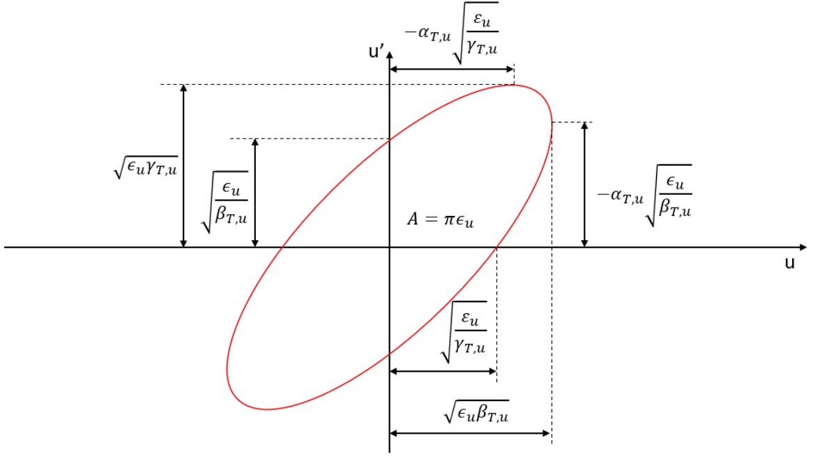
FIGURE 2.6: Elliptic area enclosing the beam in a 2D phase-space.
