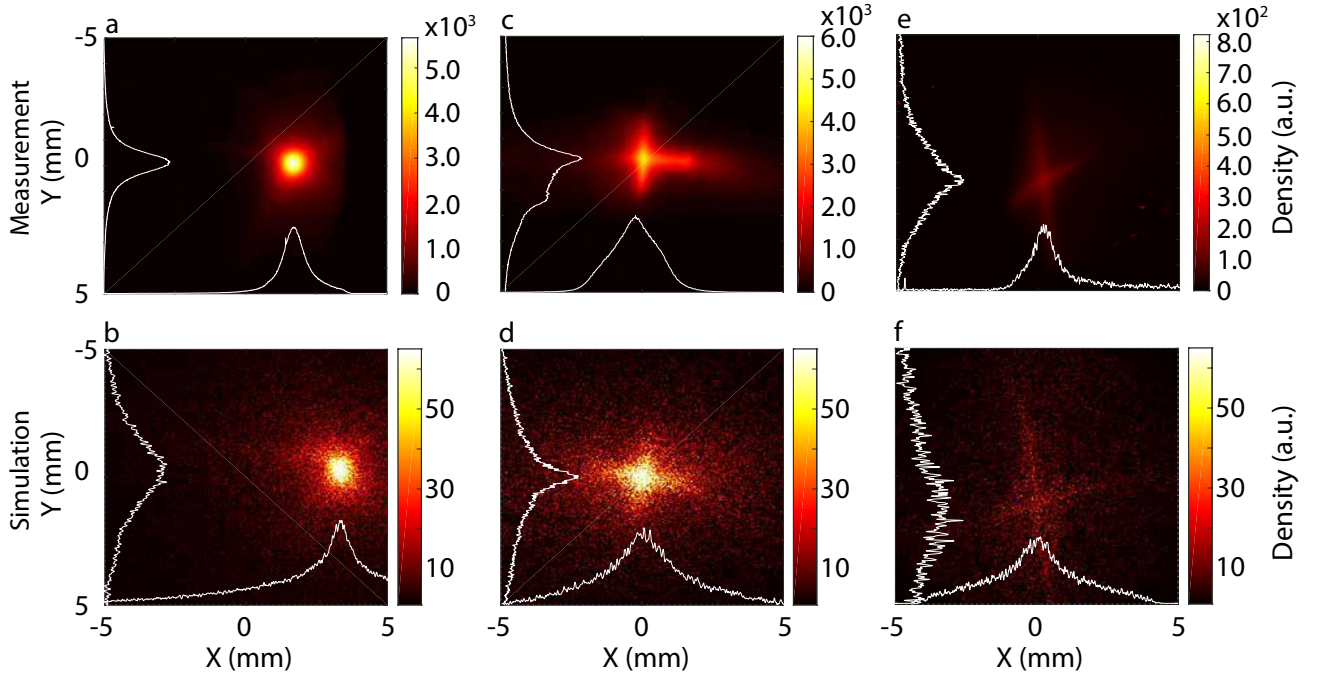
FIGURE 6.38: Transverse beam shape at the undulator entrance: measurements of RUN 3 taken the (a) 2017/03/24, (c) 2017/03/30 and (e) 2017/03/03 and simulations (b,d,f). Simulations done with the high skew a_2 case ( a_2 = 0.073, -0.325, 0.362 ; Table 3.8), \epsilon_{y,i,RMS}, \epsilon_{x,i,RMS} = 0.2 mm.mrad. (a,b) With \sigma'_{y,i,RMS} = 2 mrad, \sigma'_{x,i,RMS} = 4.7 mrad and the “Undulator entrance” optics. (c,d) With \sigma'_{y,i,RMS} = 2 mrad, \sigma'_{x,i,RMS} = 4.7 mrad and the “supermatching” optics. (e,f) With \sigma'_{y,i,RMS} = 2.5 mrad, \sigma'_{x,i,RMS} = 5.9 mrad and the “Undulator exit” optics. Shot-to-shot pointing for (a,c,e): 0.85 \pm 0.03 mrad, 0.13 \pm 0.15 mrad, and 0.07 \pm 0.02 mrad ( -0.03 \pm 0.05 mrad, -0.03 \pm 0.04 mrad, 0.18 \pm 0.04 mrad) in the horizontal (vertical) direction.
