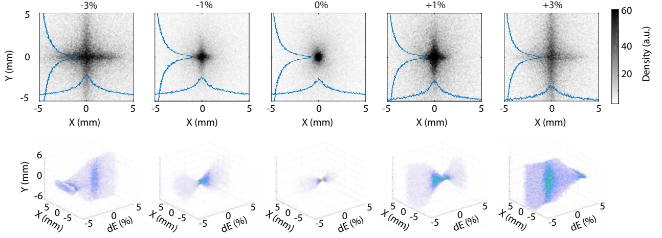
FIGURE 6.34: Electron beam transverse shape ( top ) and corresponding vertical-horizonal position per energy ( bottom ) at the undulator exit for the relative gradient change of QUAPEVA 2 of \pm 3 , \pm 1 , and 0%. Case of “undulator entrance” optics with the low divergence beam distribution (Figure 4.8c and Table 6.7), \epsilon_{x,i}, \epsilon_{y,i}, \epsilon_{y,i,RMS} = 0.2 mm.mrad, \sigma'_{y,i,RMS} = 2 mrad, \sigma'_{x,i,RMS} = 3.12 mrad [178].
