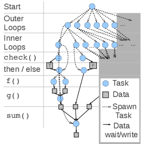
Figure 4.3: Example of Swift code
