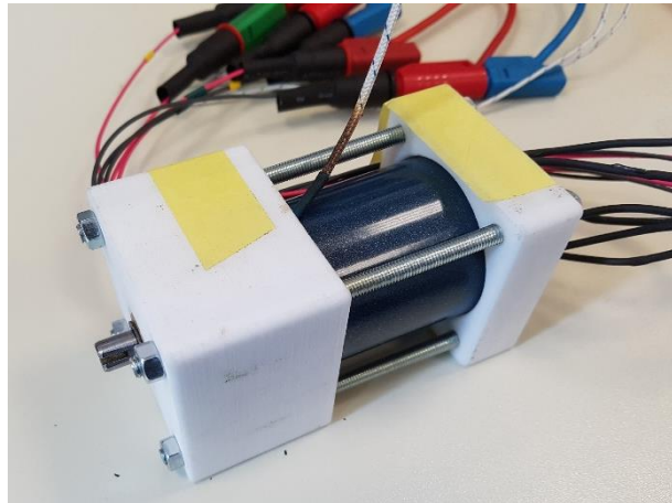
Figure II-34 : Prototype 6s4p16barres
