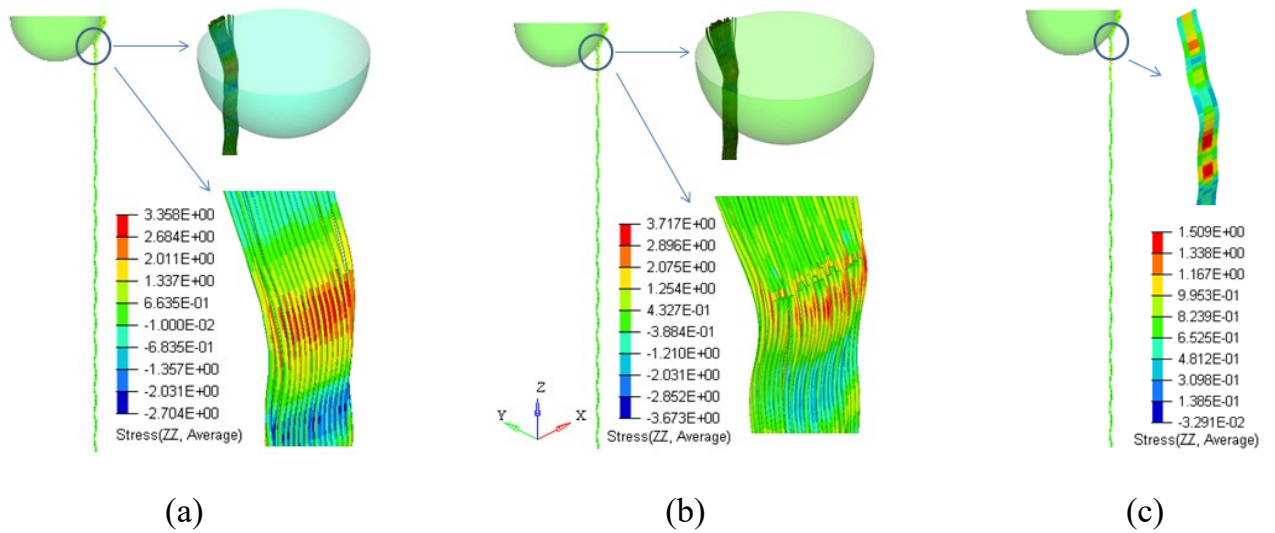
Figure IV.8 Deformation at 2.1 \mu s (a) 42-fibres (b) 98-fibres (c) mesoscopic model.
