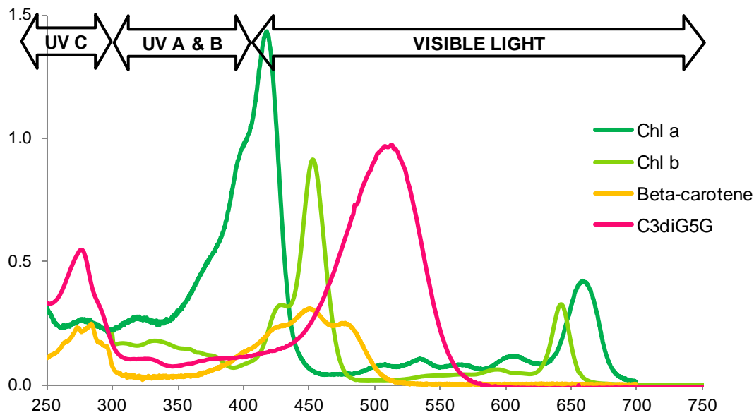
Fig. 1. Absorption spectra of natural pigments: the photosynthetic chlorophylls a and b; the accessory pigment \beta -carotene and the non-photosynthetic cyanidin-3,5-diglucoside (spectral data from Taniguchi, 2001 & Li, 1997)
