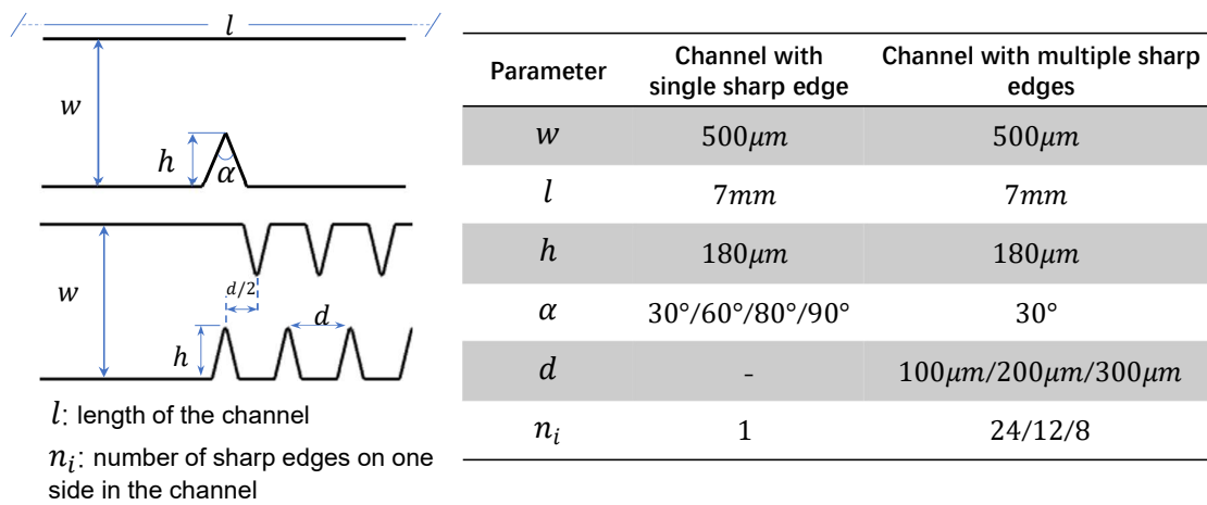
Figure 2.2 – Sharp-edge geometries in different steps of the study
