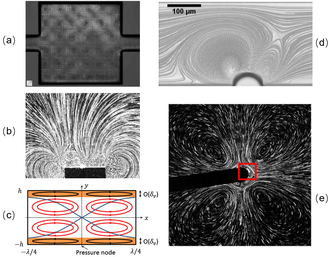
Figure 1.4 – Rayleigh streaming under different acoustic or mechanical forcing and with different geometries: (a) acoustic streaming in a square PDMS microchamber at f = 2.17\text{MHz} BRUUS [2007] ; (b) streaming flow around a vibrating metal beam inserted into the water/glycerine solution, f = 200\text{Hz} COSTALONGA et collab. [2015] ; (c) schematic presentation of a streaming flow in a two-dimensional rectangular channel LEI et collab. [2017] ; (d) streaming flow around an acoustically excited bubble in a microchannel at f = 16.8\text{kHz} WANG et collab. [2012] ; (e) streaming flow around a vibrating cylinder immersed within a fluid at f = 60\text{Hz} , the vortex contained by the red square mark refers to the inner streaming within the viscous boundary layer, and the area out of the layer is dominated by the outer streaming or Rayleigh streaming BAHRANI et collab. [2020]
