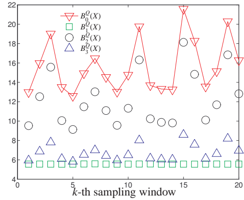
Figure 5.11: Efficient scores in these 20 sampling windows
