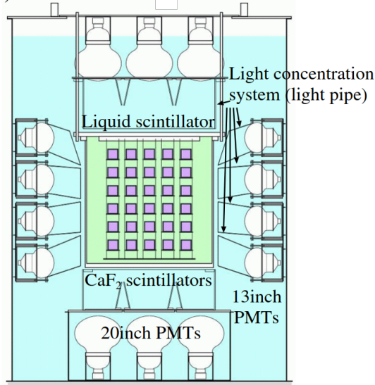
Figure 1.14: Sketch of the CANDLES detector.
