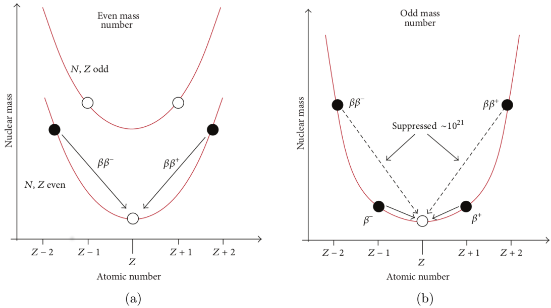
Figure 1.6: Nuclear mass as a function of the atomic number Z in the case of an isotope with A even (a) and A odd (b). Adapted from [11].
