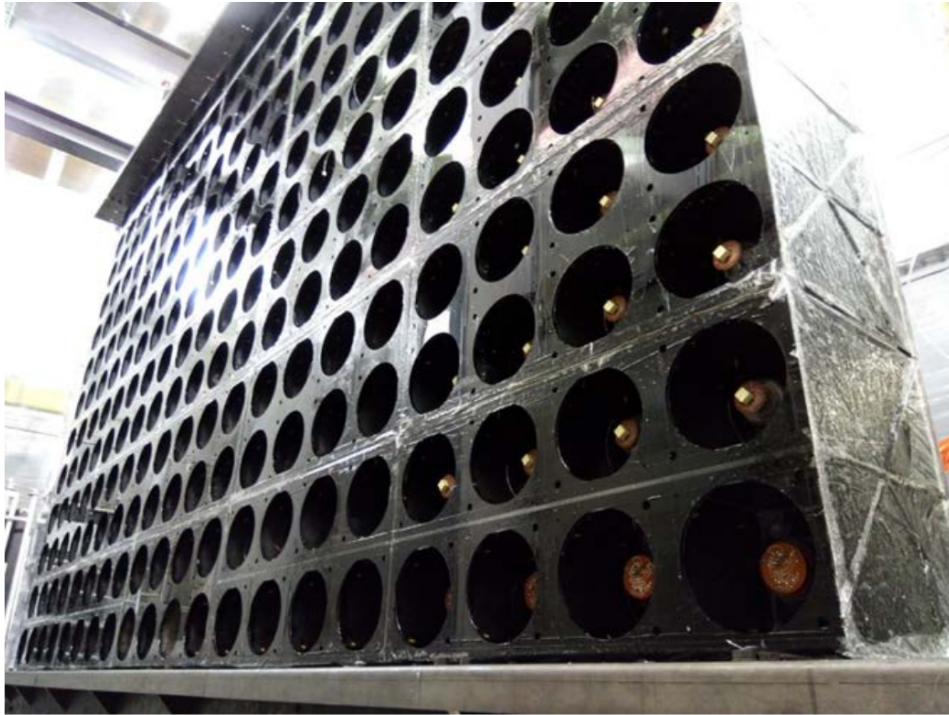
(a) Back view of one calorimeter main wall.
