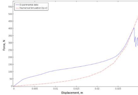
Figure 5.12: Comparison between the experimental measurements of reaction force for a pantographic structure with quasi-perfect pivots (blue) and the numerical simulation for a structure with perfect pivots (red, dot-dashed). The numerical simulation is lower than the experimental measure.
