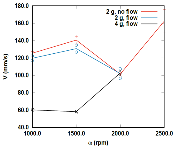
(a) Q_3(V)
