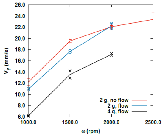
(c) Q_3(V_y)
