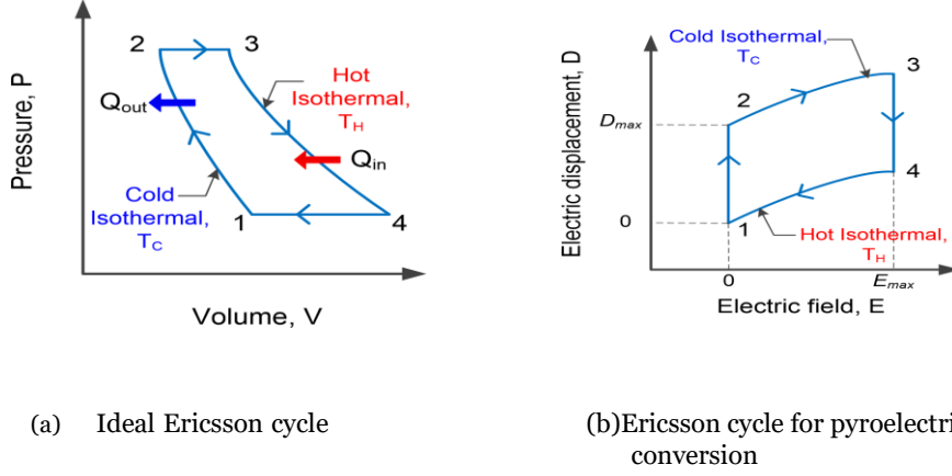
Figure 2.17 Ericsson cycles.
