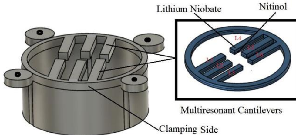
Figure 3. 23 Schematic of the proposed multi resonant piezoelectric energy harvester
