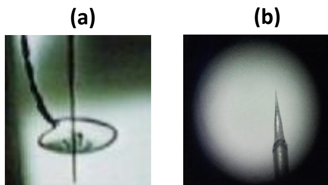
Fig. 2.3: Preparation method of an STM tip: (a) Electrochemical etching of a tungsten (W) piece with a NaOH solution (10%). (b) Real photo of an STM Tip.
