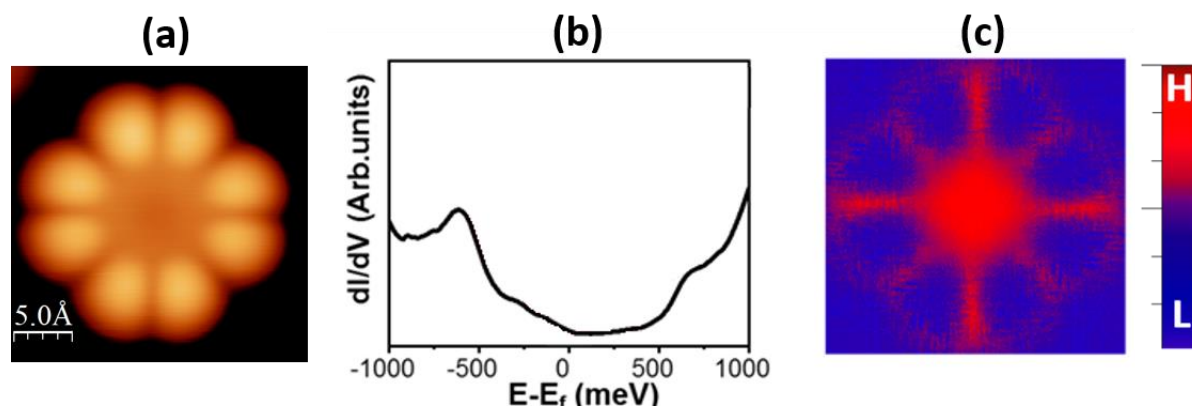
Fig. 2.12: Example of experimental results obtained by STM/STS on TbPc_2 deposited on Cu(111). (a) Topographic STM image of TbPc_2 . (b) Conductance spectrum ( dI/dV ) acquired at the center revealing the HOMO and LUMO states. (c) dI/dV maps at occupied states (-0.7 V). Red: high conductance, blue: low conductance.
