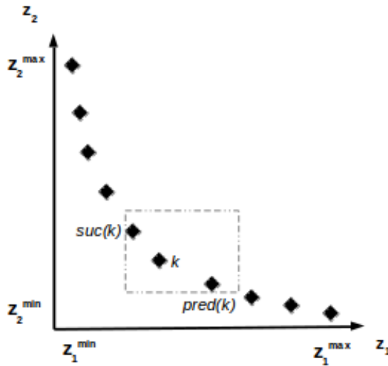
FIGURE 6.2 – Distance de crowding
