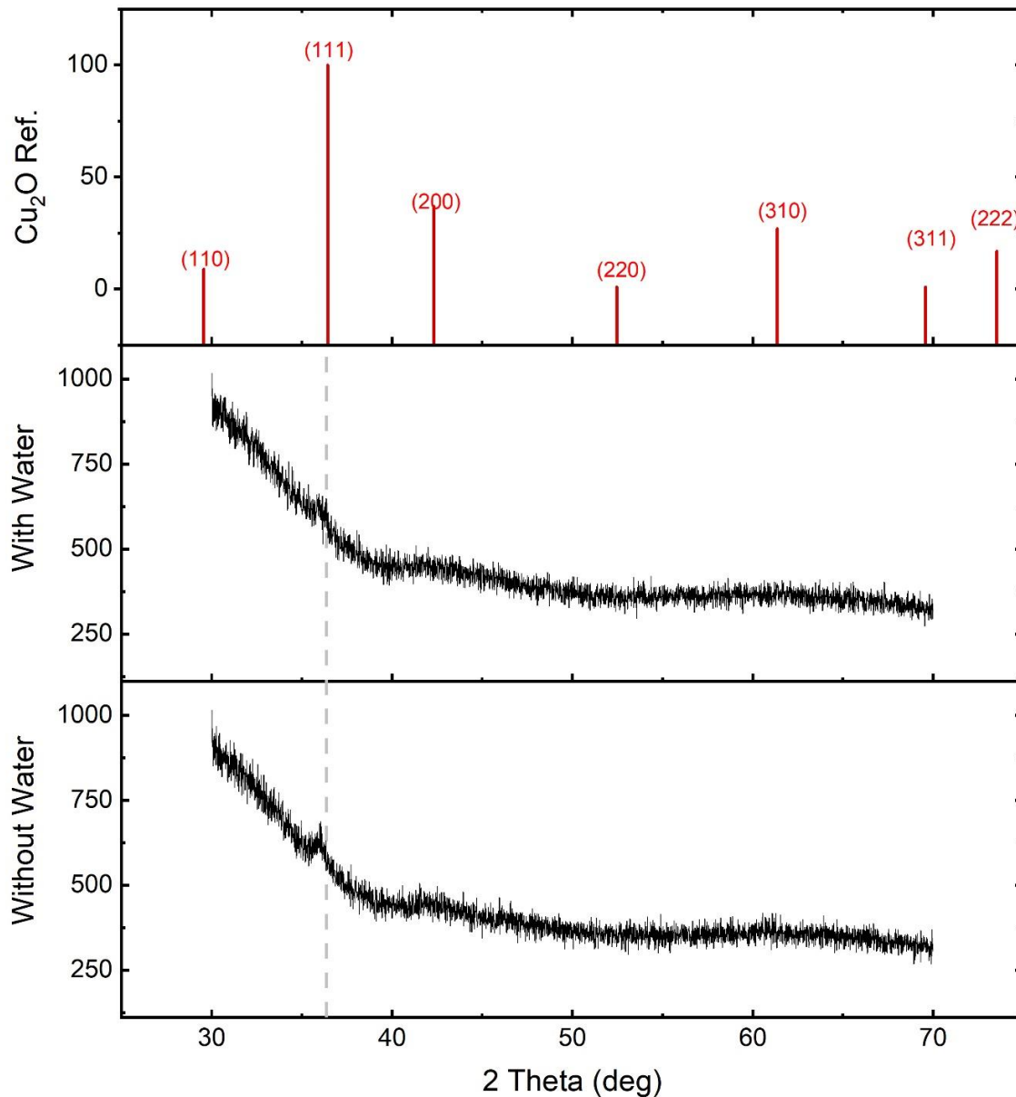
Figure 5-36. XRD patterns of Cu 2 O films deposited with 15% oxygen and 83% water (a) and 15% oxygen and 0% water.
