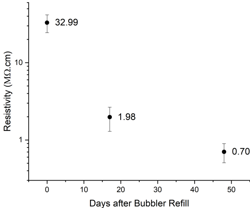
Figure 5-14. Resistivity as a function of the time that has passed after the Cupraselect bubbler was refilled.
