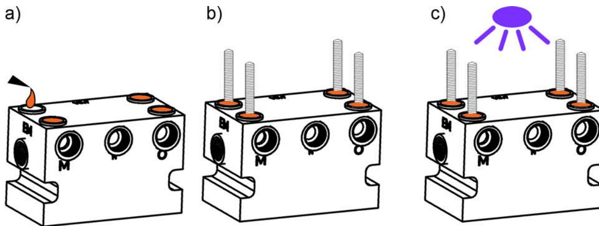
Figure 4-11. Schematic of the process for the fixation of the screws on the deposition head. a) A drop of liquid resin is inserted in the required place. b) The screws are submerged in the liquid resin, taking care to hold them as straight as possible. c) Exposition to UV light for 15 to 30 minutes, depending on the amount and type of resin used.
