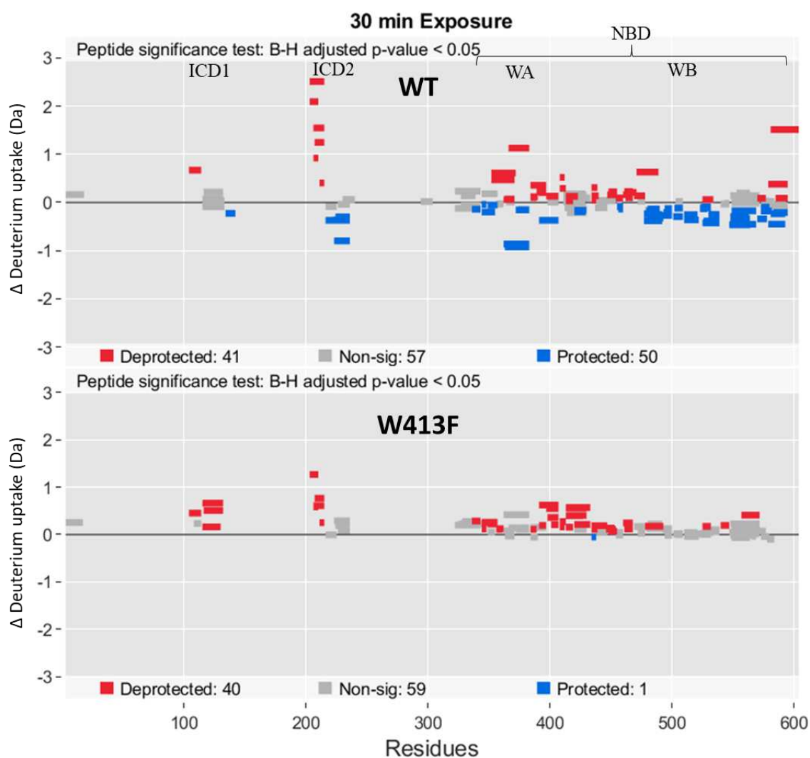
Fig 65. Differential HDX plot of WT and W413F BmrA in nanodiscs between the Apo and doxorubicin-bound (100 \mu M doxo) conditions at 30 min D 2 O exposure. Blue signifies the peptides protected against deuteration in doxo-bound condition, whereas red signifies the deprotected peptides. Grey represents peptides having p-value more than 0.05. All measurements were done in duplicate except for WT apo.
