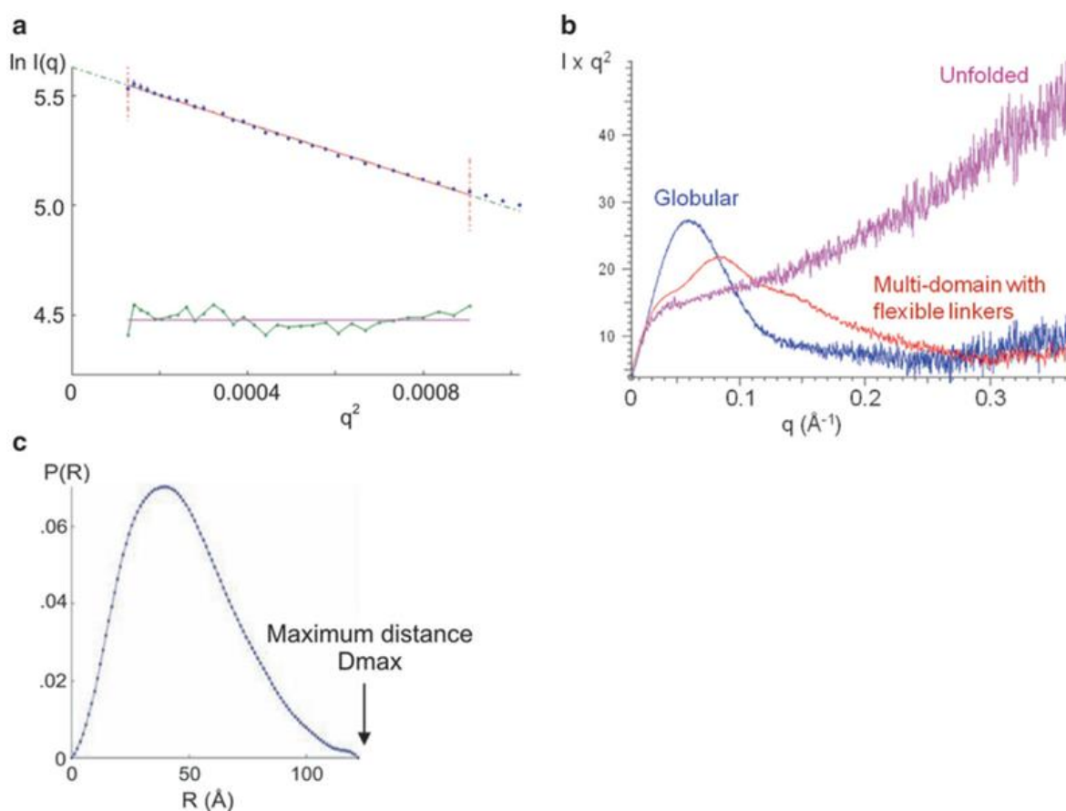
Fig 31. SANS primary data analysis. (a) Guinier plot is shown with the fit of the Guinier equation shown in red. The slope of the Guinier plot is used to calculate the radius of gyration. (b) Kratky plot showing characteristic curves for different types of proteins. (c) Distance distribution function p(r) . The shape of the curve shown here is asymmetric with a tailing profile at higher distances, indicative of an elongated shape of the protein (modified from (Choi & Morais, 2014)).
