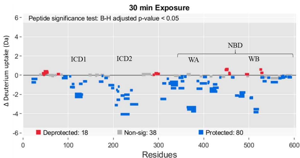
Fig 47. Differential HDX plot of WT BmrA in nanodiscs between the Apo and Vi-trapped condition at 30 min D2O exposure. Blue signifies the peptides protected against deuteration in Vi-trapped condition, whereas red signifies the deprotected peptides. Grey represents peptides with p-value more than 0.05. All measurements were done in duplicate.
