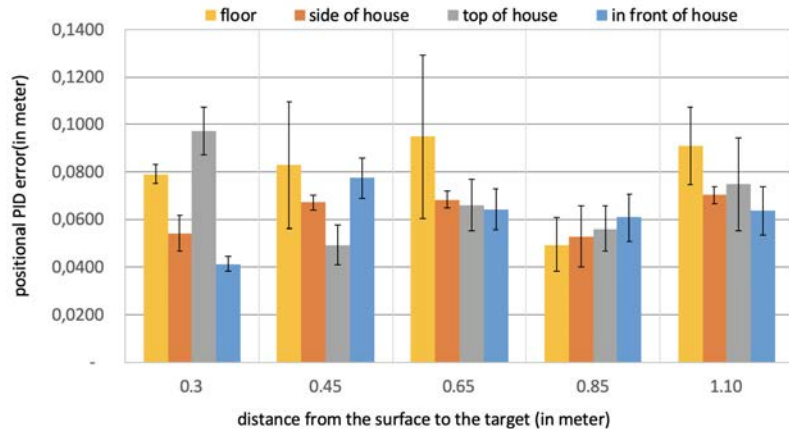
Figure 4.20: The drone positioning error to the target locations for all four surfaces. Overall error is 6.8 \pm 1.1\text{cm} .
