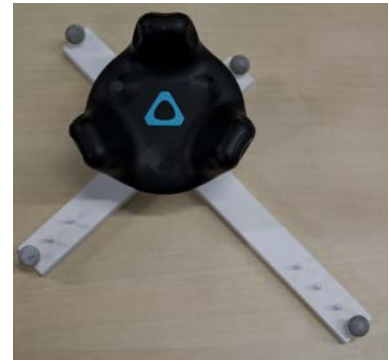
Figure 4.16: A HTC vive tracker with retro reflective markers.
