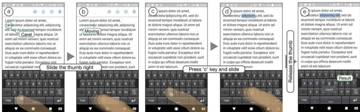
Figure 3.7: Usage of Press & Slide technique [167].
