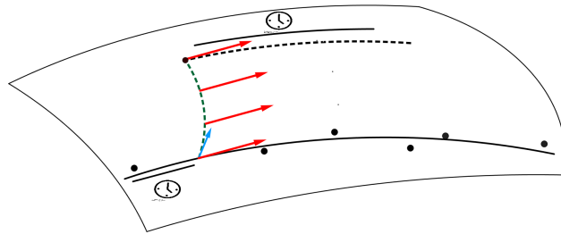
Figure 3.2: Reparametrized geodesic parallelization. Matching time and exp-parallel trajectory are reparametrized.
