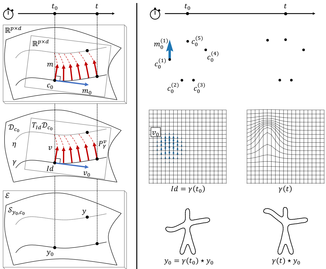
Figure 4.1: [Left] . Shape spatiotemporal reference frame y_0, c_0, m_0, t_0 with respect to which a shape y admits coordinates t \in \mathbb{R}, v \in v_0^\perp \subset T_{\gamma(t_0)}\mathcal{D}_{c_0} . Three spaces are involved: the manifold of control points \mathbb{R}^{p \times d} , the manifold of diffeomorphisms \mathcal{D}_{c_0} , and the shape submanifold \mathcal{S}_{y_0, c_0} of the extrinsic shape space \mathcal{E} . The momenta m_0, m and the velocity fields v_0, v are in one-to-one correspondence. The velocity field v , also called space-shift, is parallel-transported along the geodesic \gamma by the operator t \rightarrow P_\gamma^v(t) . Figure 4.2 illustrates the effect of parallel transport on \mathcal{D}_{c_0} .
