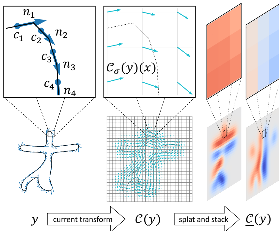
Figure 7.1: Current-splating mechanics. The input mesh is first transformed in a vector field, which is then discretized on a fixed grid to form a d -dimensional image. If a topologically simple object was selected for the sake of clarity, note that any other topology could be similarly treated.
