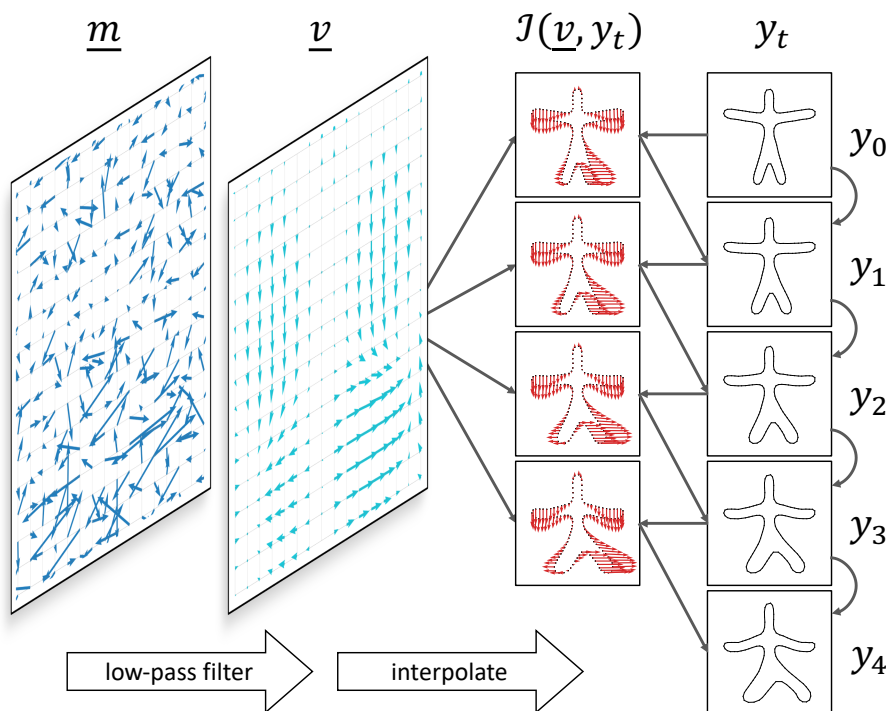
Figure 7.2: Exponentiation mechanics. The input d -dimensional array \underline{m} is first filtered by a Gaussian convolution layer. Interpreted as a discretized velocity field, the resulting \underline{v} is interpolated on the successive positions of the moving mesh y_t , which is finally updated accordingly.
