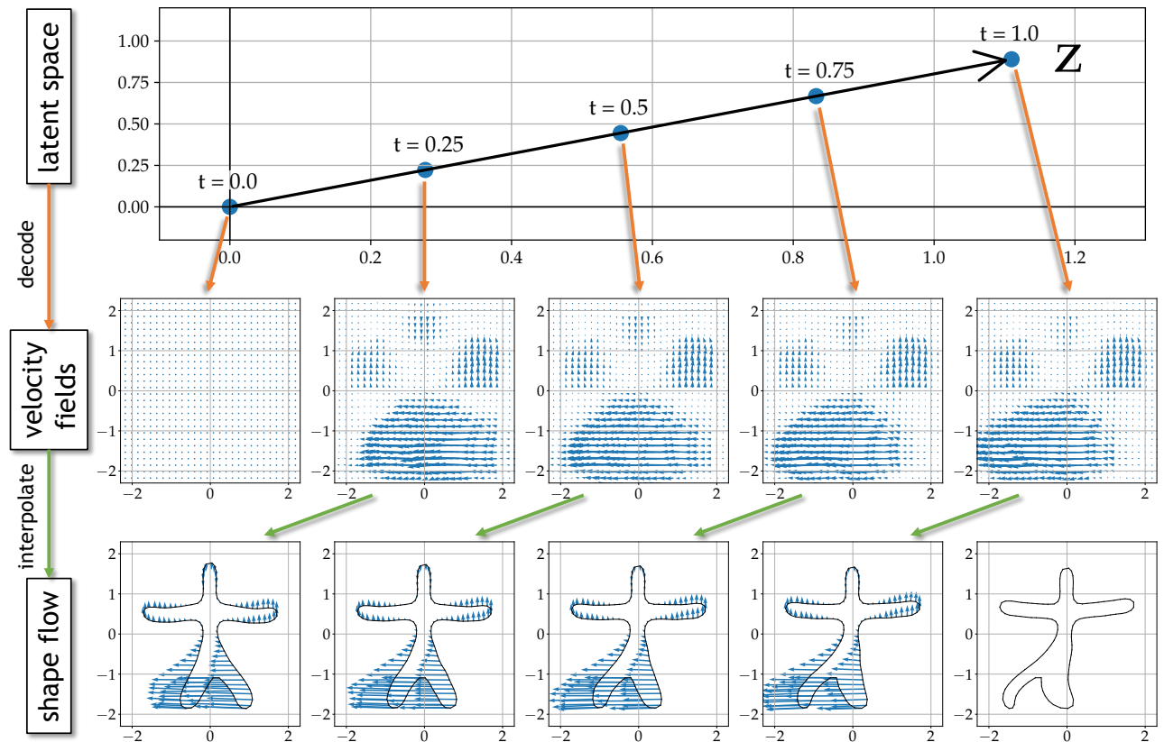
Figure 9.1: Deformation mechanics: diffeomorphisms are obtained by following the streamlines of dynamic velocity fields, which are themselves defined as the image of latent-space segments by a non-linear mapping represented in practice by a network. The parameters of this decoding mapping will be optimized for each new application, therefore adapting the core deformation mechanics to the considered data set.
