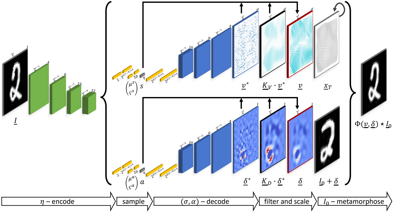
Figure 8.2: Architecture of the metamorphic auto-encoder. The input image I is encoded by four convolution layers (in green), followed by two parallel pairs of fully-connected layers (in yellow). The encoder outputs are interpreted as characterizing two normal distributions, from which are sampled the latent codes s \in \mathbb{R}^p and a \in \mathbb{R}^q . Two parallel decoders successively composed of two fully connected and four deconvolution layers map those latent shape and appearance representations to the velocity field v^* and intensity increment \delta^* duals. After filtering by the operators K_V and K_D , the obtained vectors are explicitly scaled, enforcing the equality of their Hilbert norm with the Euclidean norm of the corresponding codes s and a . The resulting velocity field v and intensity increment \delta are finally combined to metamorphose the prototype image parameter I_0 (see Figure 8.1).
