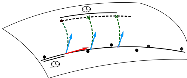
Figure 3.4: Reparametrized exp-parallelization. Matching time and exp-parallel trajectory are reparametrized.
