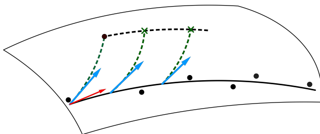
Figure 3.3: Exp-parallelization. Red arrow: geodesic regression. Blue arrows: transported baseline matching. Black dotted line : exp-parallelization of the reference geodesic for the given subject.
