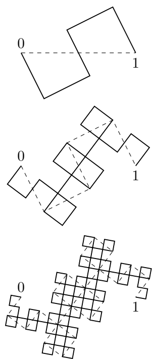
Construction of the (+1, +1, +1, -1, +1) -Koch curve.
